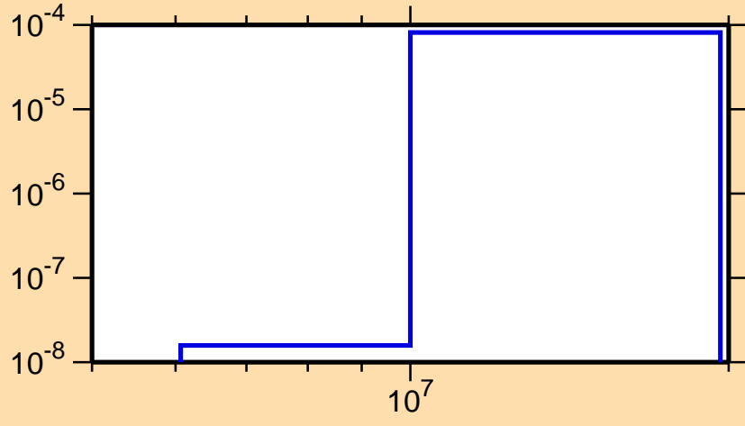
\sigma vs. E for ^{252}\text{No}(\text{mt } 45)
