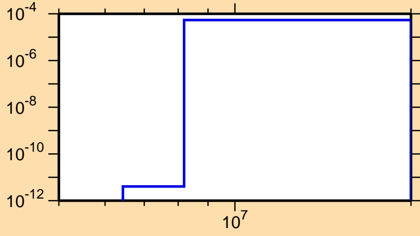
\sigma vs. E for ^{252}\text{No}(\text{mt117})
