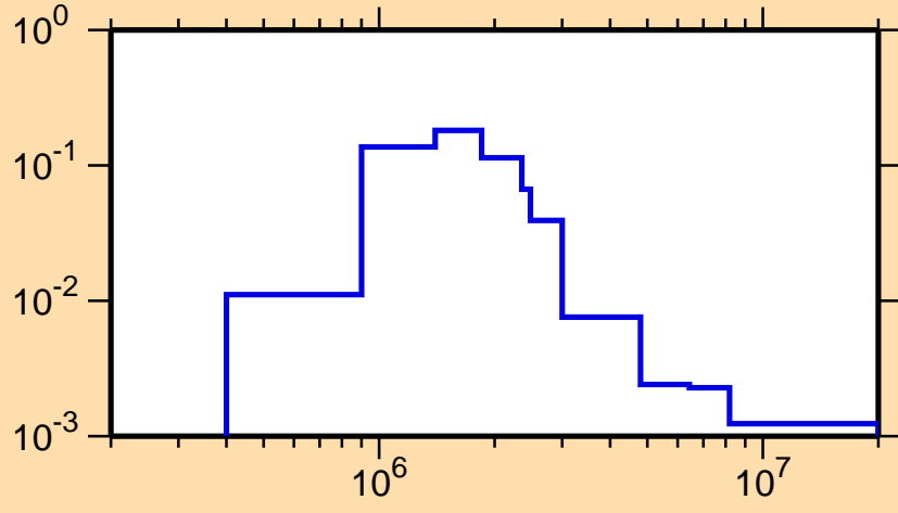
\sigma vs. E for ^{252}\text{No}(n,n_3)
