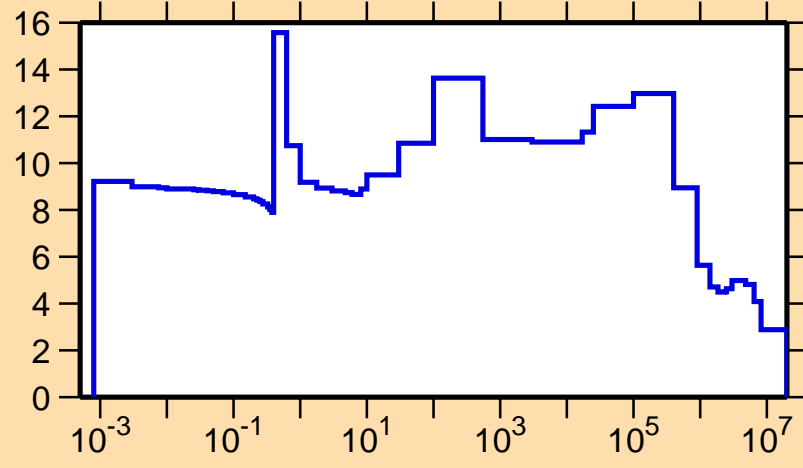
\sigma vs. E for ^{252}\text{No}(n,\text{el.})
