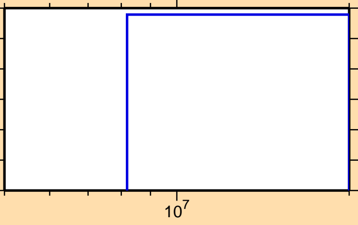
\sigma vs. E for ^{252}\text{No}(n,\text{nd})
