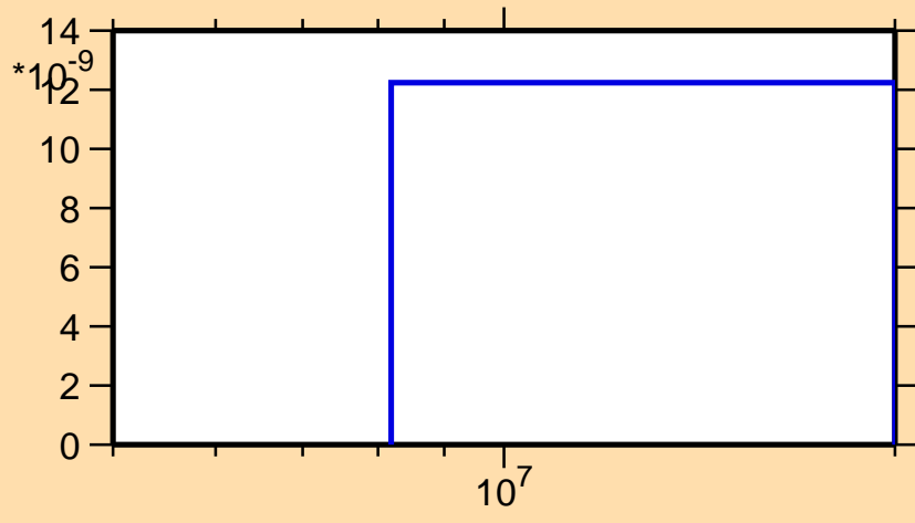
\sigma vs. E for ^{252}\text{No}(n,2np)
