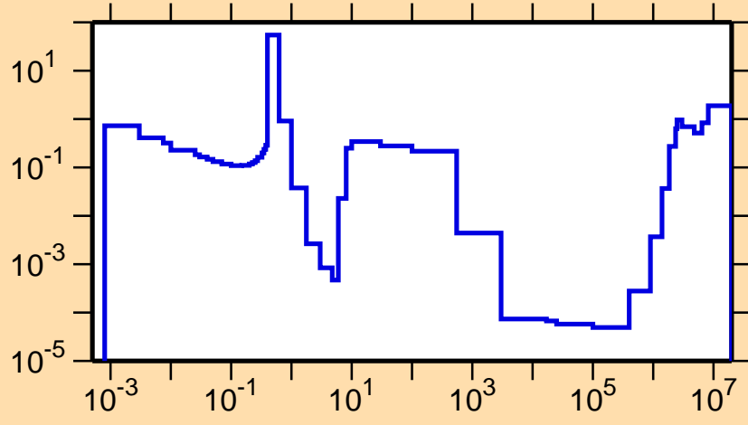
\sigma vs. E for ^{252}\text{No}(n,f)
