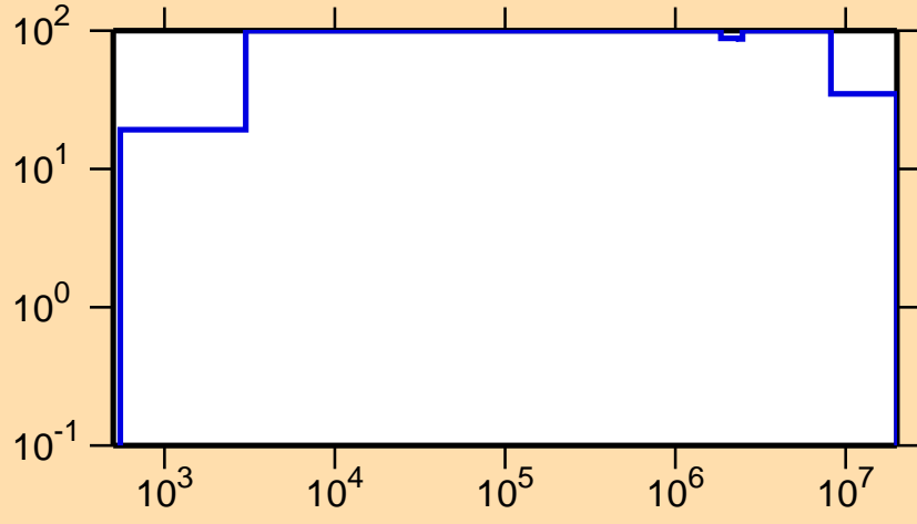
\Delta\sigma/\sigma vs. E for ^{252}\text{No}(n,f)
