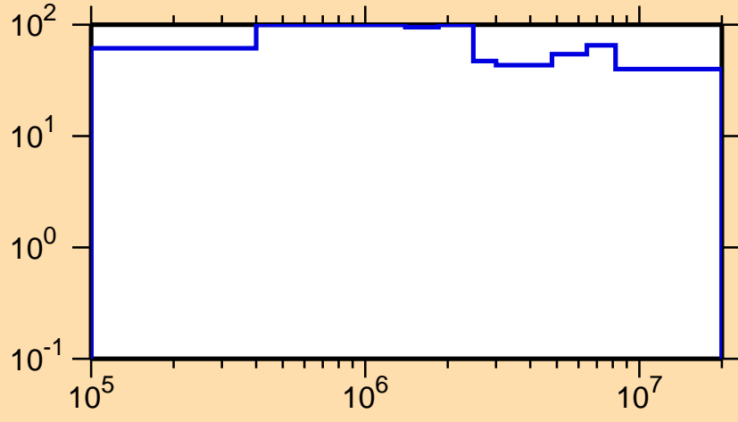
\Delta\sigma/\sigma vs. E for ^{252}\text{No}(n,n\text{cont.})
