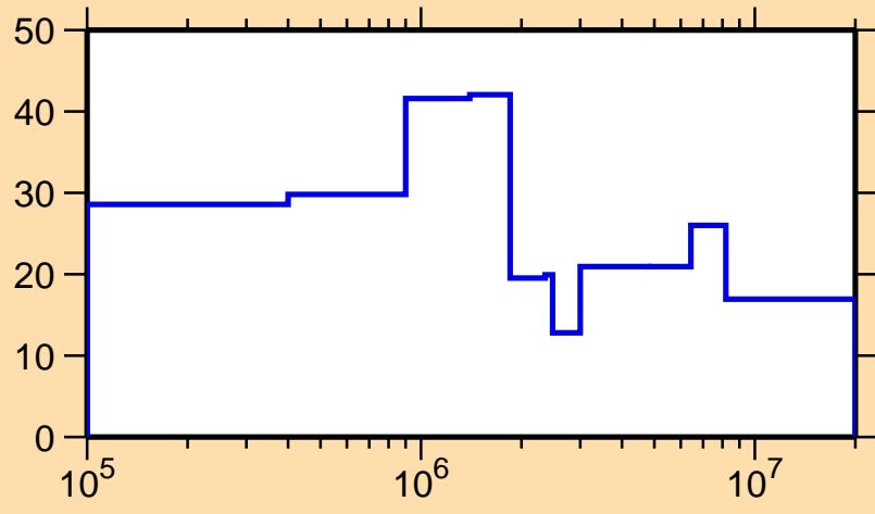
\Delta\sigma/\sigma vs. E for ^{252}\text{No}(n,\text{el.})
