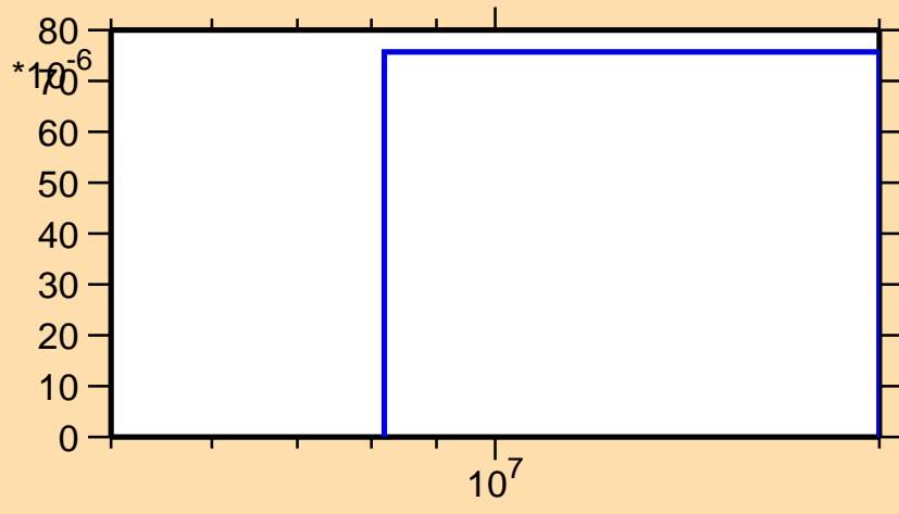
\sigma vs. E for ^{252}\text{No}(n,3n\alpha)
