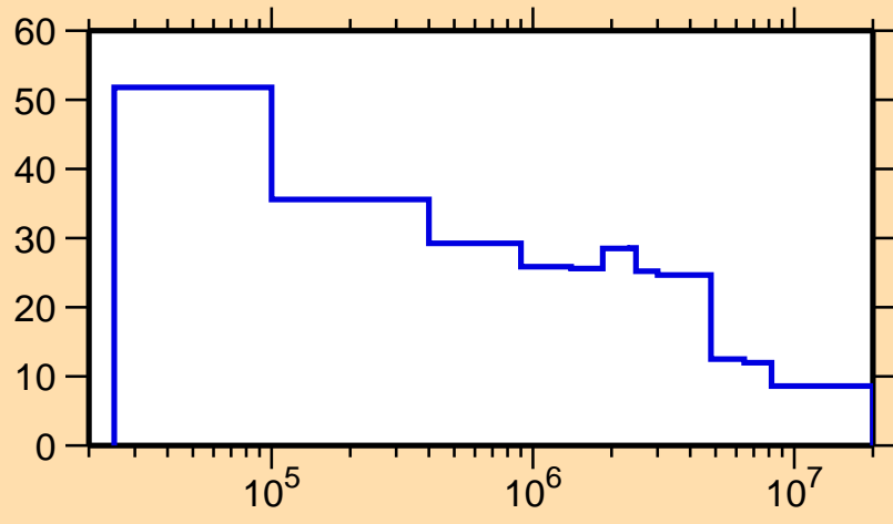
\Delta\sigma/\sigma vs. E for ^{252}\text{No}(n,\text{nonel.})
