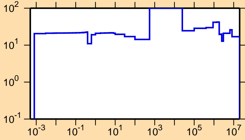
\Delta\sigma/\sigma vs. E for ^{252}\text{No}(n,el.)
