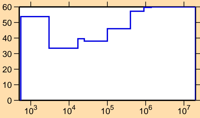
\Delta\sigma/\sigma vs. E for ^{252}\text{No}(n,\gamma)
