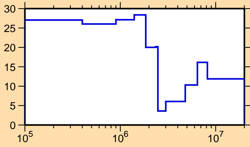
\Delta\sigma/\sigma vs. E for ^{252}\text{No}(n,\text{tot.})
