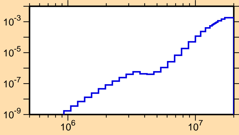
\sigma vs. E for ^{253}\text{No}(n,p\alpha)
