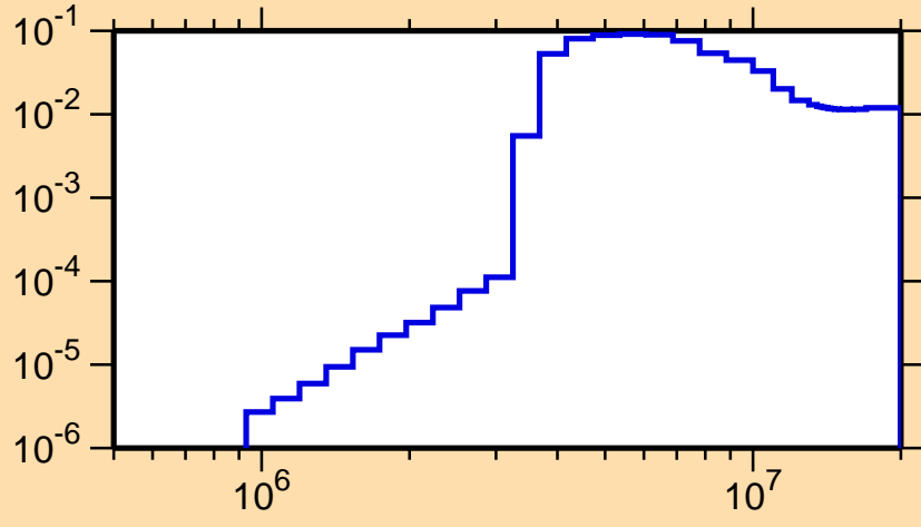
\sigma vs. E for ^{253}\text{No}(n,n\alpha)
