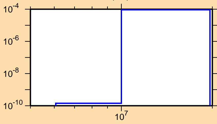
\sigma vs. E for ^{253}\text{No}(n,t)
