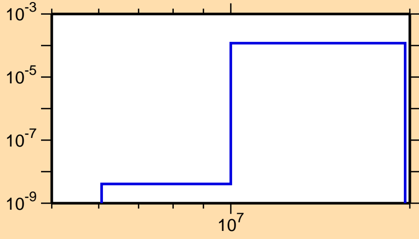
\sigma vs. E for ^{253}\text{No}(\text{mt117})
