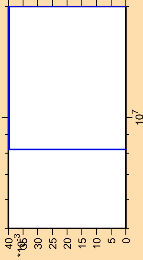
\Delta\sigma/\sigma vs. E for ^{253}\text{No}(n,\text{pt})
