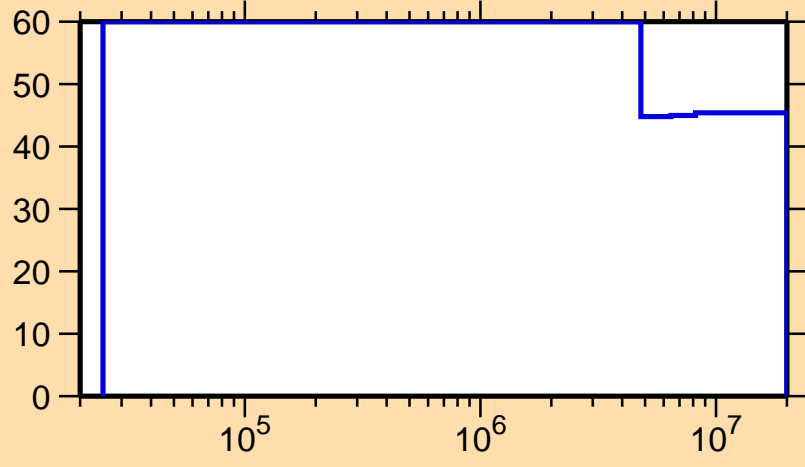
\Delta\sigma/\sigma vs. E for ^{253}\text{No}(n,n_1)
