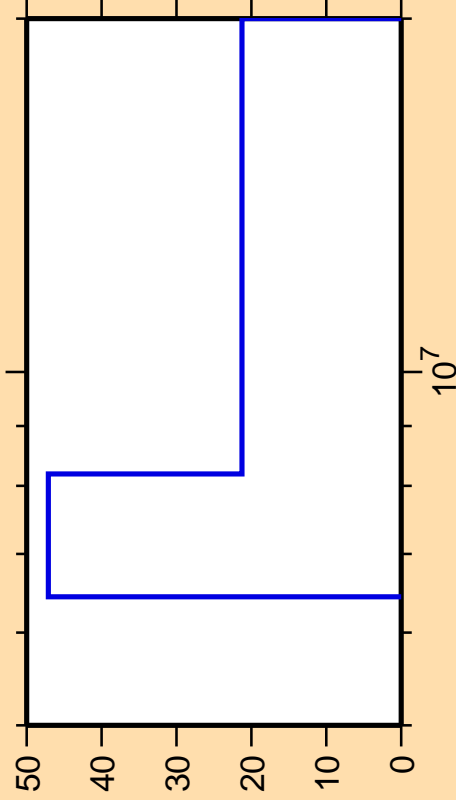
\Delta\sigma/\sigma vs. E for ^{253}\text{No}(n,d)
