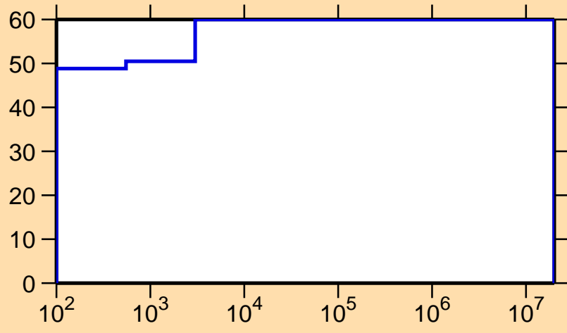
\Delta\sigma/\sigma vs. E for ^{253}\text{No}(n,\gamma)
