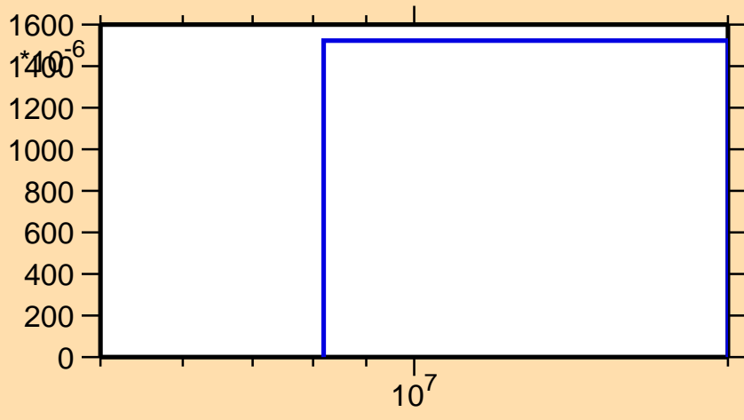
\sigma vs. E for ^{253}\text{No}(n,3n)
