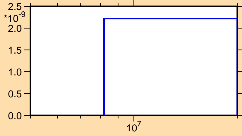
\sigma vs. E for ^{253}\text{No}(n,\text{He3})
