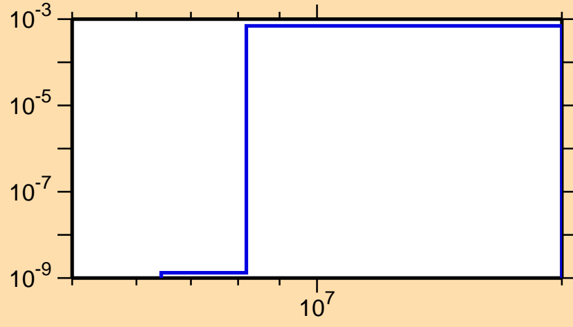
\sigma vs. E for ^{253}\text{No}(n,d)
