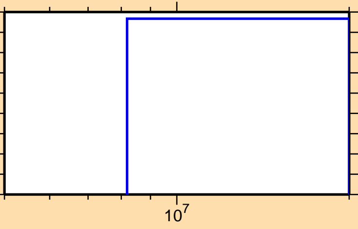
\sigma vs. E for ^{253}\text{No}(n,nt)
