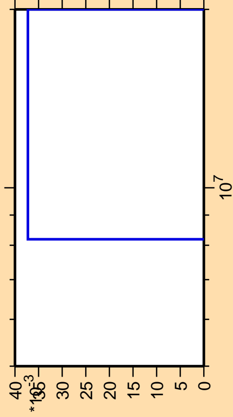
\Delta\sigma/\sigma vs. E for ^{253}\text{No}(n,\text{pd})
