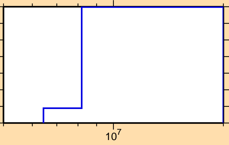
\sigma vs. E for ^{253}\text{No}(\text{mt117})
