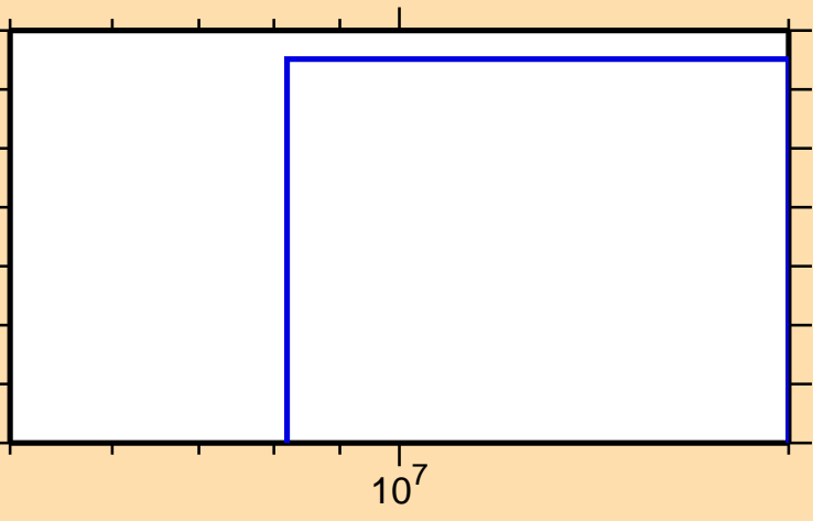
\sigma vs. E for ^{253}\text{No}(n,\text{nd})
