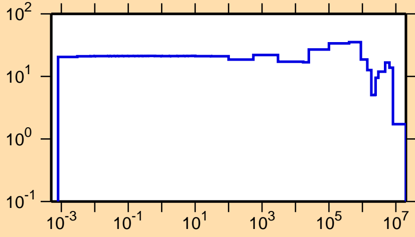
\Delta\sigma/\sigma vs. E for ^{253}\text{No}(n,el.)
