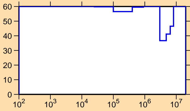
\Delta\sigma/\sigma vs. E for ^{253}\text{No}(n,p)
