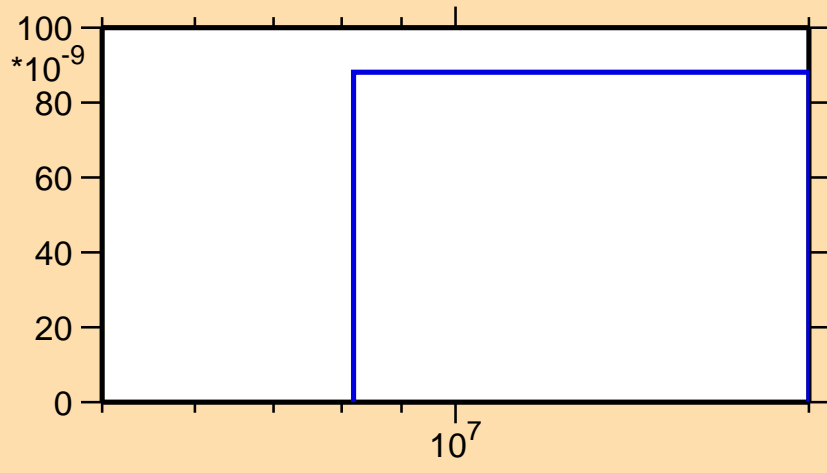
\sigma vs. E for ^{253}\text{No}(n,2np)
