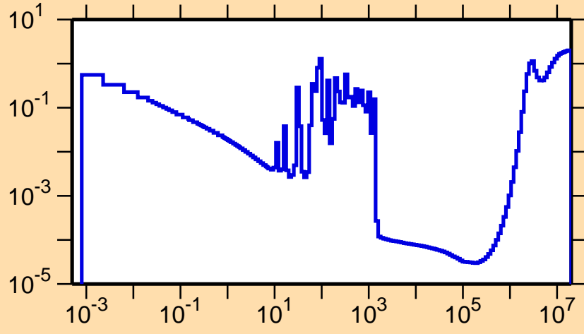
\sigma vs. E for ^{254}\text{No}(n,f)
