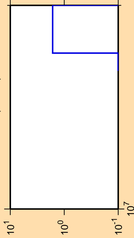
\Delta\sigma/\sigma vs. E for ^{254}\text{No}(\text{mt } 34)
