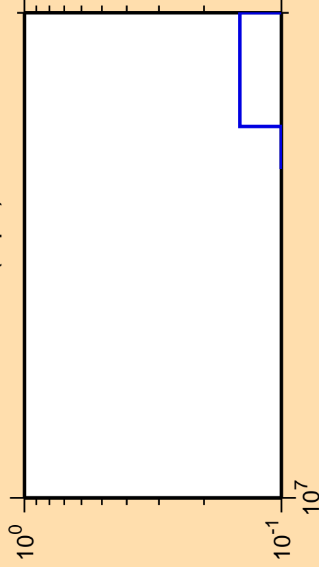
\Delta\sigma/\sigma vs. E for ^{254}\text{No}(n,\text{pd})
