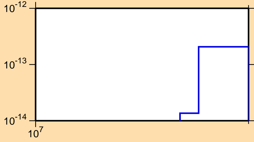
\sigma vs. E for ^{254}\text{No}(n,\text{pd})
