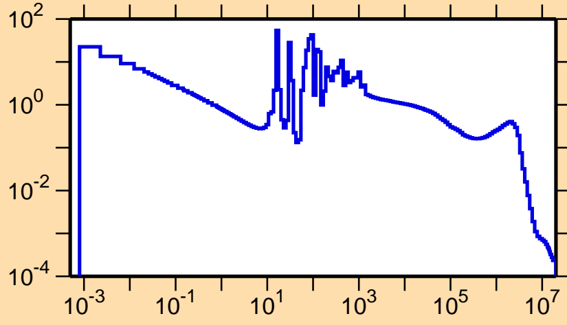
\sigma vs. E for ^{254}\text{No}(n,\gamma)
