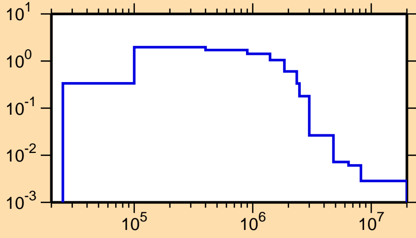
\sigma vs. E for ^{254}\text{No}(n,n_1)
