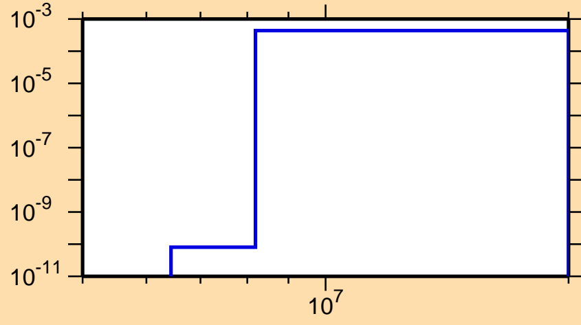
\sigma vs. E for ^{254}\text{No}(n,d)
