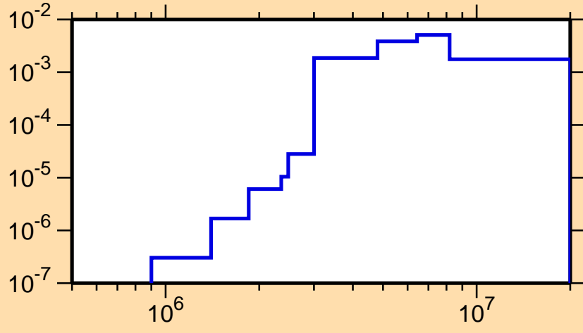
\sigma vs. E for ^{254}\text{No}(n,n\alpha)
