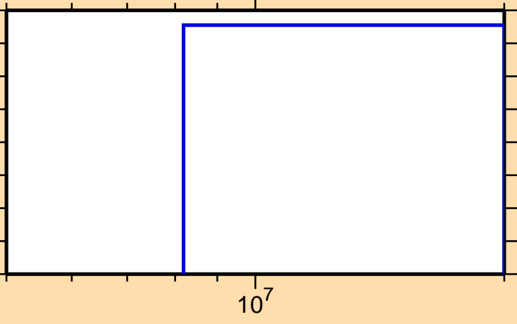
\sigma vs. E for ^{254}\text{No}(n,\text{nd})
