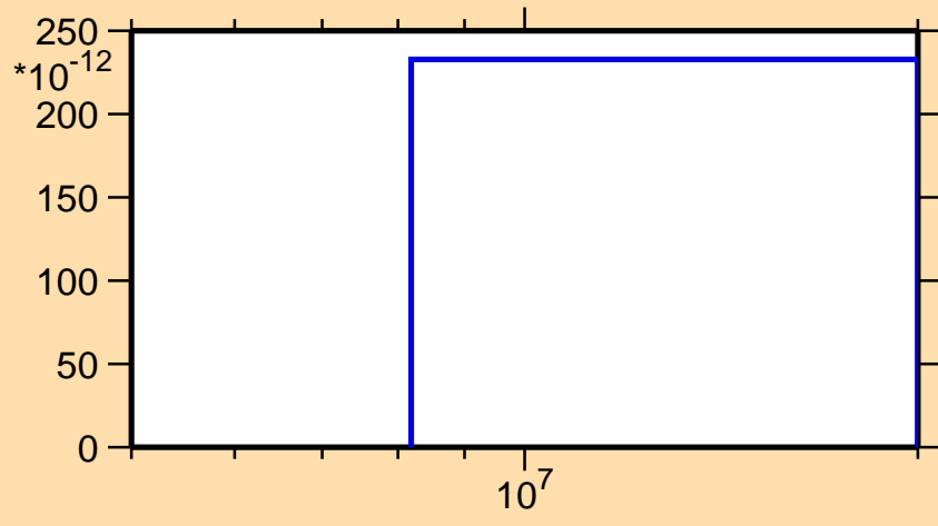
\sigma vs. E for ^{254}\text{No}(n,\text{He3})
