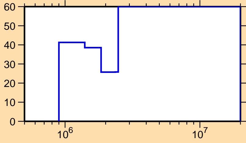
\Delta\sigma/\sigma vs. E for ^{254}\text{No}(n,\gamma)
