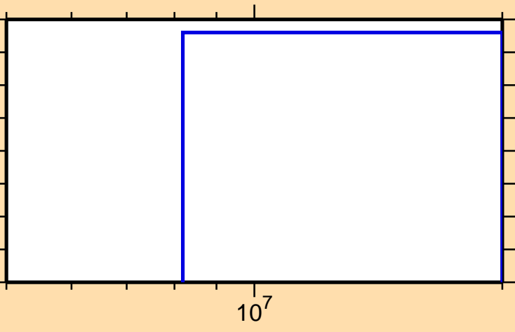
\sigma vs. E for ^{254}\text{No}(n,3n\alpha)
