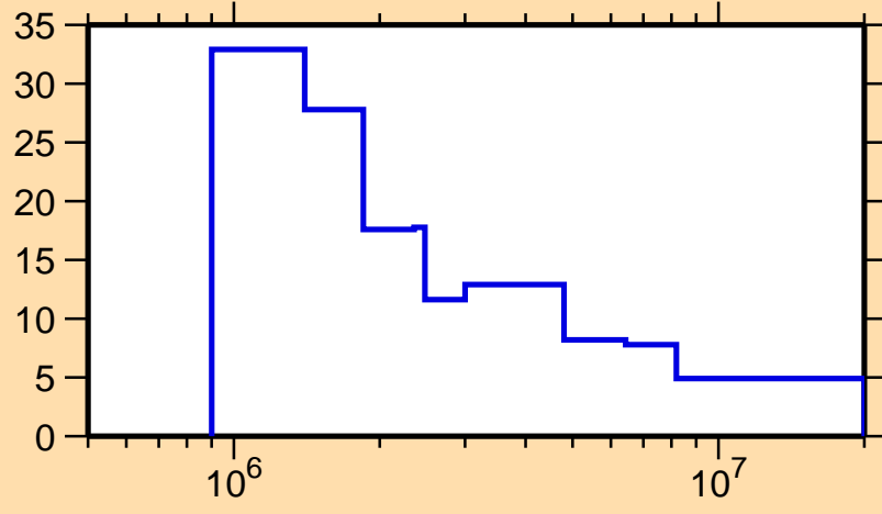
\Delta\sigma/\sigma vs. E for ^{254}\text{No}(n,\text{nonel.})
