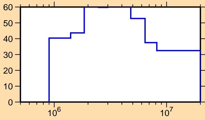
\Delta\sigma/\sigma vs. E for ^{254}\text{No}(n,n_1)
