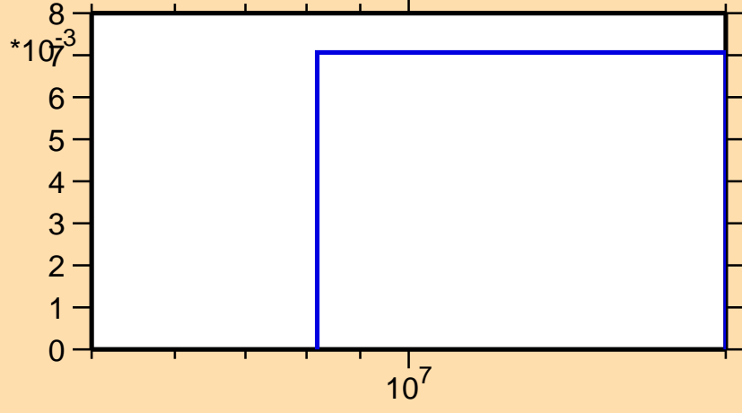
\sigma vs. E for ^{254}\text{No}(n,3n)
