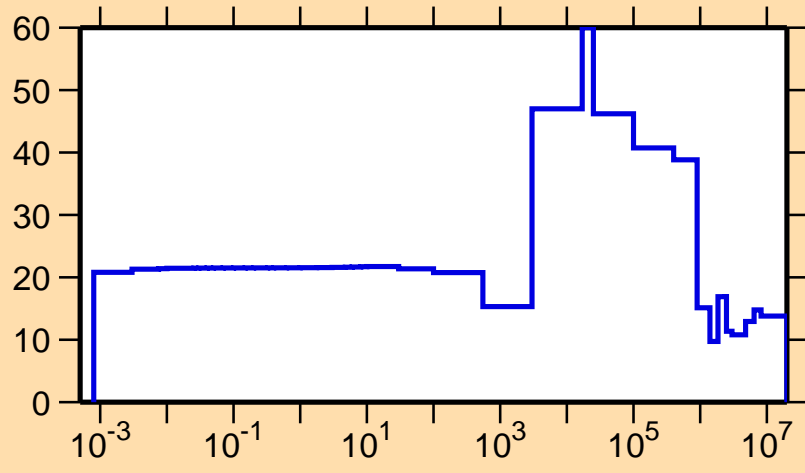
\Delta\sigma/\sigma vs. E for ^{254}\text{No}(n,el.)
