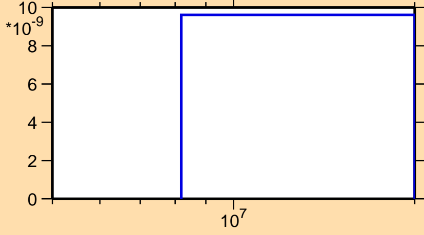
\sigma vs. E for ^{254}\text{No}(n,2np)
