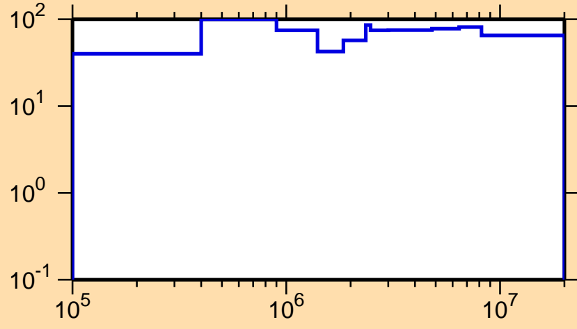
\Delta\sigma/\sigma vs. E for ^{254}\text{No}(n,n\text{cont.})
