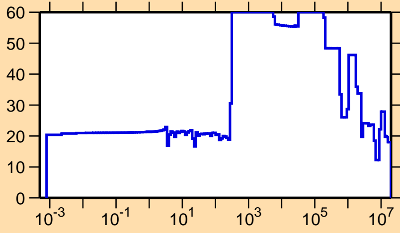
\Delta\sigma/\sigma vs. E for ^{255}\text{No}(n,el.)
