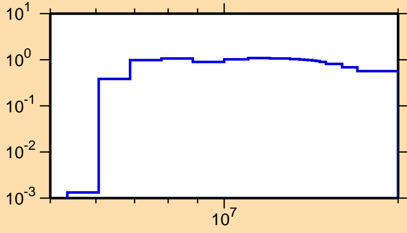
\sigma vs. E for ^{255}\text{No}(n,2n)
