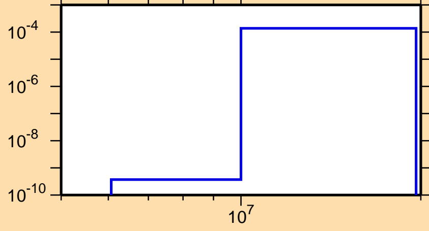
\sigma vs. E for ^{255}\text{No}(n,t)
