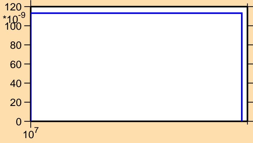
\sigma vs. E for ^{255}\text{No}(n,\text{nd})
