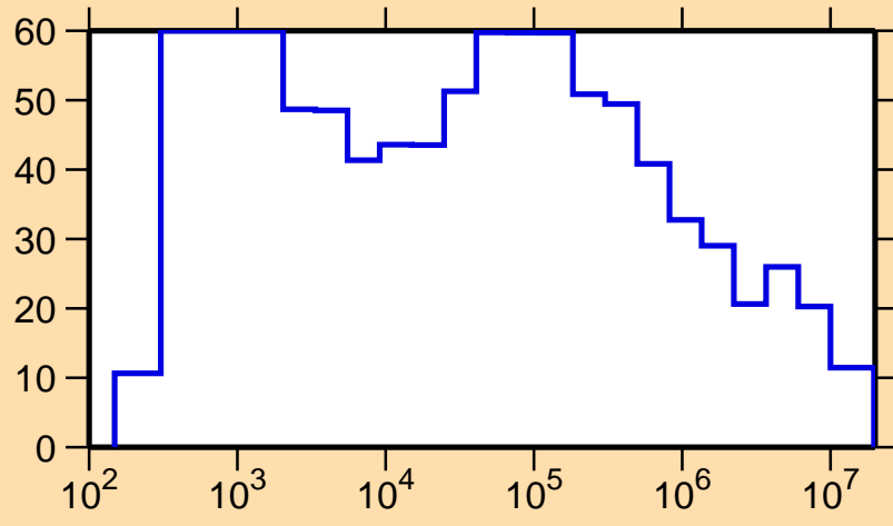
\Delta\sigma/\sigma vs. E for ^{255}\text{No}(n,\text{tot.})
