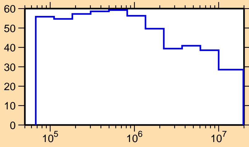
\Delta\sigma/\sigma vs. E for ^{255}\text{No}(n,\text{nonel.})
