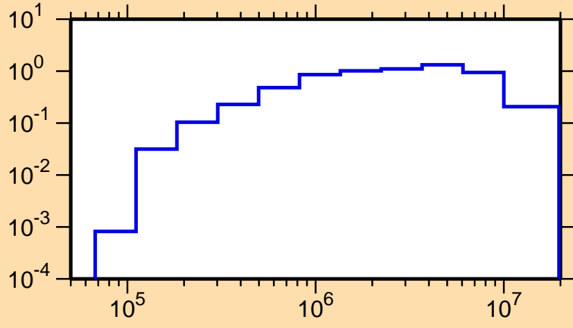
\sigma vs. E for ^{255}\text{No}(n,n\alpha)
