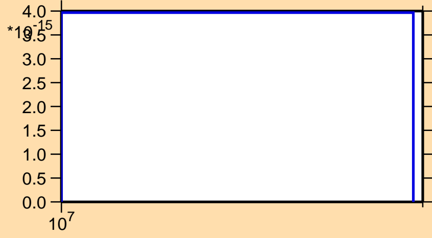
\sigma vs. E for ^{255}\text{No}(n,\text{pt})
