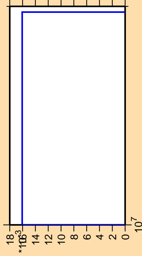
\Delta\sigma/\sigma vs. E for ^{255}\text{No}(n,\text{pt})
