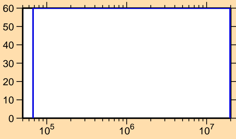
\Delta\sigma/\sigma vs. E for ^{255}\text{No}(n,\text{inel.})
