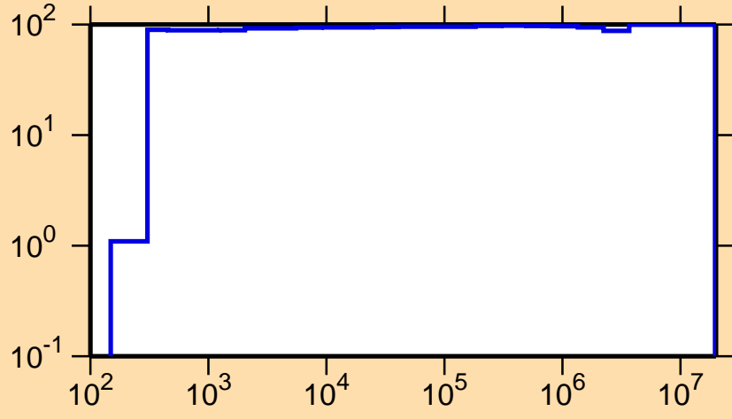
\Delta\sigma/\sigma vs. E for ^{255}\text{No}(n,\gamma)
