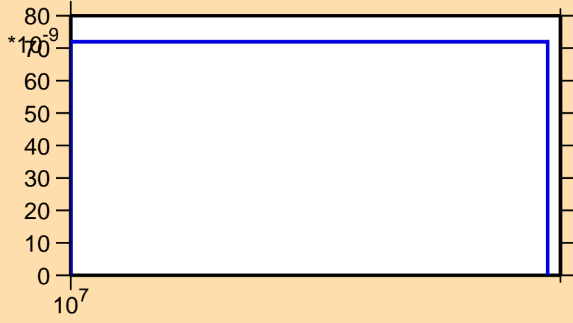
\sigma vs. E for ^{255}\text{No}(n,2np)
