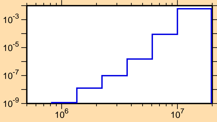
\sigma vs. E for ^{255}\text{No}(n,p)
