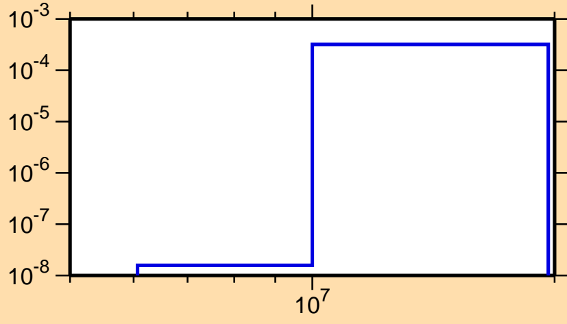
\sigma vs. E for ^{255}\text{No}(n,np)
