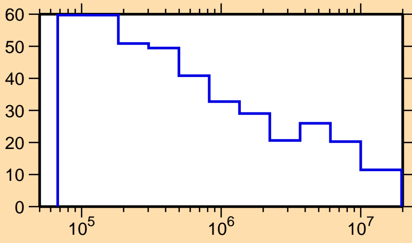
\Delta\sigma/\sigma vs. E for ^{255}\text{No}(n, tot.)
