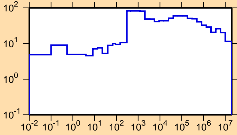
\Delta\sigma/\sigma vs. E for ^{255}\text{No}(n,\text{tot.})
