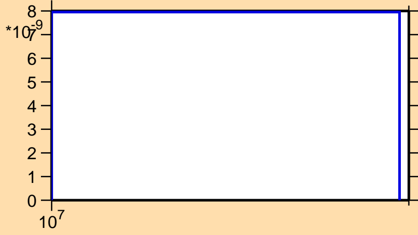
\sigma vs. E for ^{255}\text{No}(n,nt)
