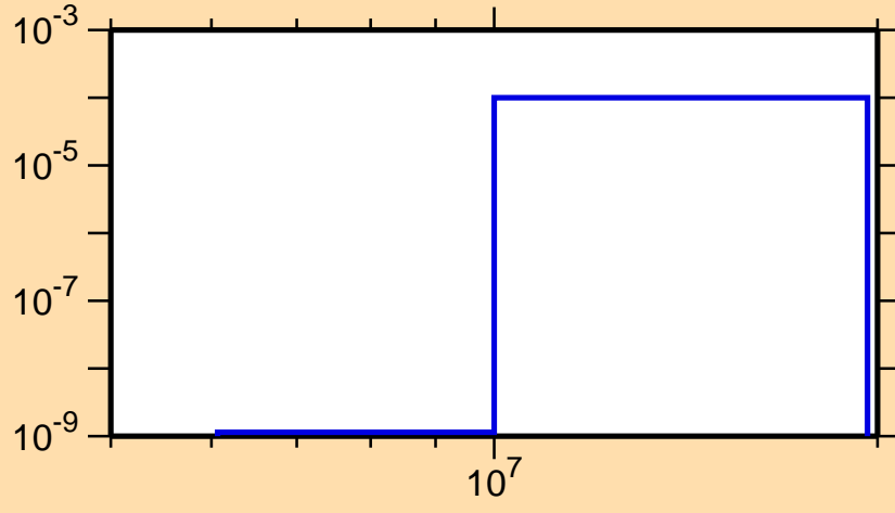
\sigma vs. E for ^{255}\text{No}(\text{mt117})
