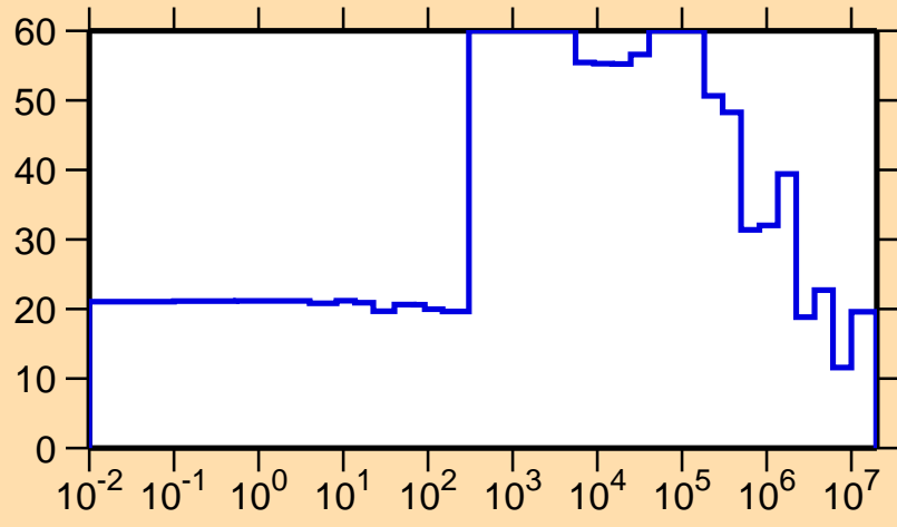
\Delta\sigma/\sigma vs. E for ^{255}\text{No}(n,\text{el.})
