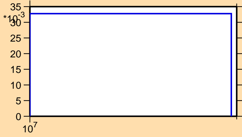
\sigma vs. E for ^{255}\text{No}(n,3n)
