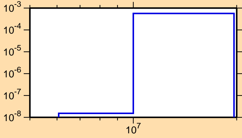
\sigma vs. E for ^{255}\text{No}(n,d)
