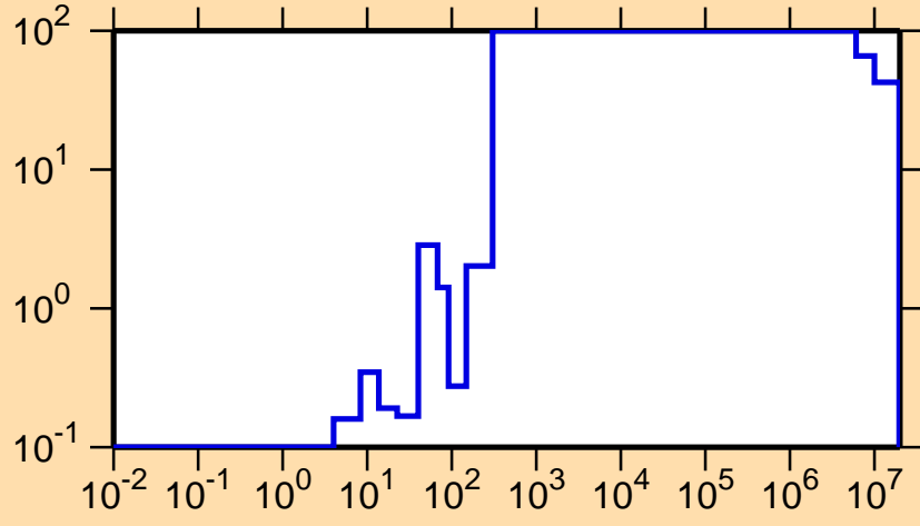
\Delta\sigma/\sigma vs. E for ^{255}\text{No}(n,f)
