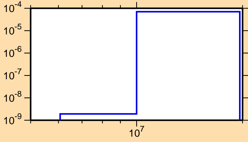
\sigma vs. E for ^{255}\text{No}(\text{mt } 45)
