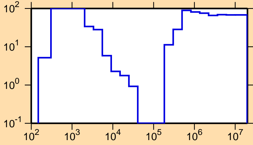
\Delta\sigma/\sigma vs. E for ^{255}\text{No}(n,p)
