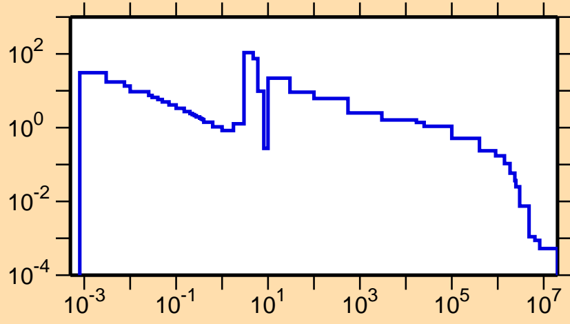
\sigma vs. E for ^{255}\text{No}(n,\gamma)
