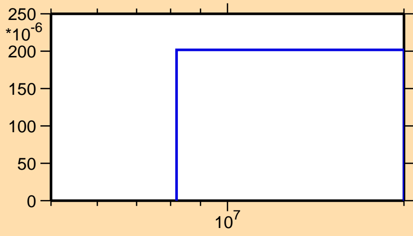
\sigma vs. E for ^{255}\text{No}(n,3n\alpha)
