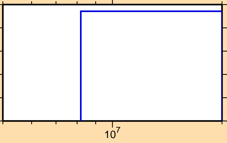
\sigma vs. E for ^{255}\text{No}(n,\text{nd})
