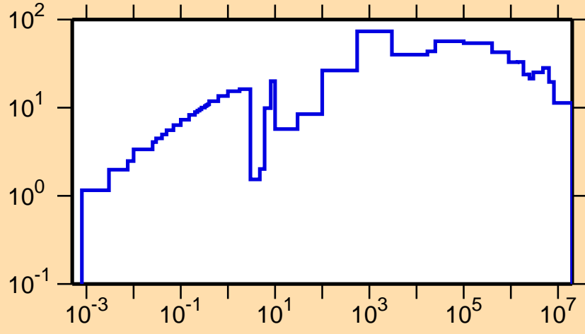
\Delta\sigma/\sigma vs. E for ^{255}\text{No}(n,tot.)
