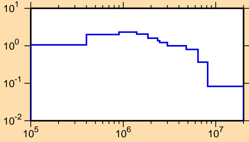
\sigma vs. E for ^{255}\text{No}(n,\text{inel.})
