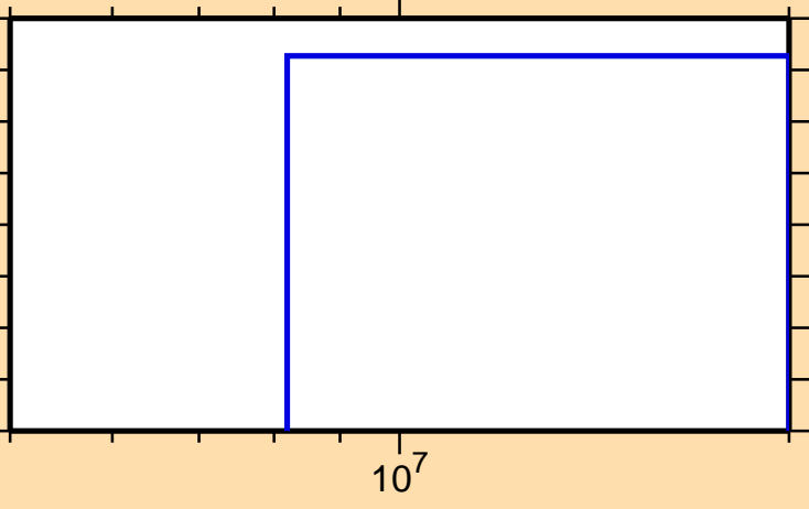
\sigma vs. E for ^{255}\text{No}(n,nt)
