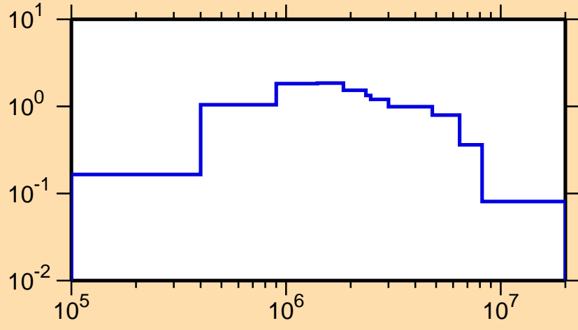
\sigma vs. E for ^{255}\text{No}(n,n\text{cont.})
