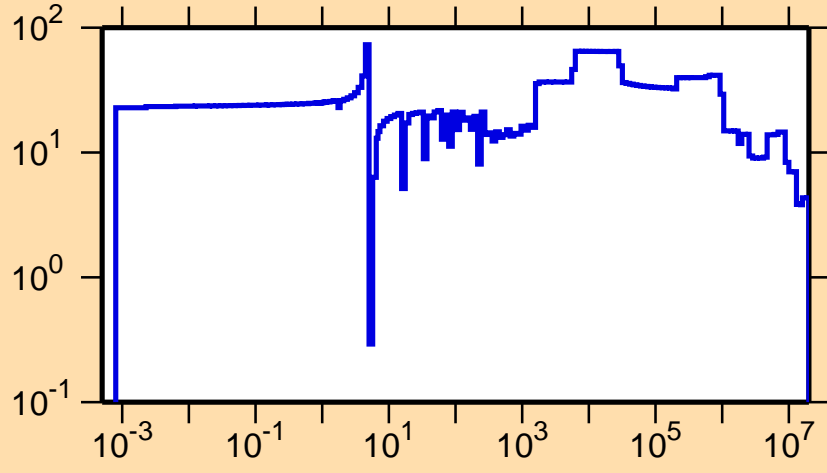
\Delta\sigma/\sigma vs. E for ^{256}\text{No}(n,el.)
