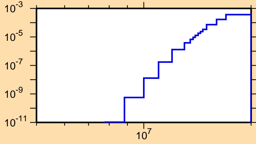
\sigma vs. E for ^{256}\text{No}(\text{mt117})
