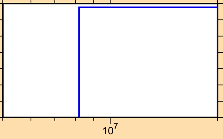
\sigma vs. E for ^{257}\text{No}(n,nt)
