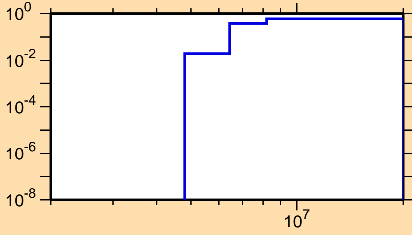
\sigma vs. E for ^{257}\text{No}(n,2n\alpha)
