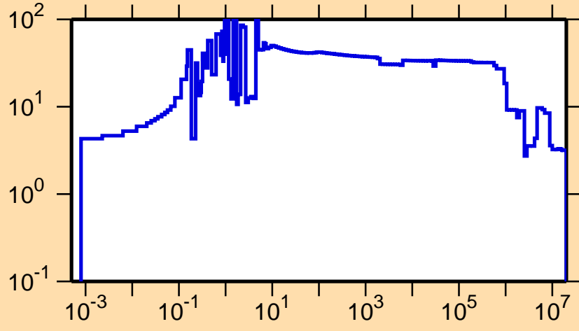
\Delta\sigma/\sigma vs. E for ^{259}\text{No}(n,tot.)
