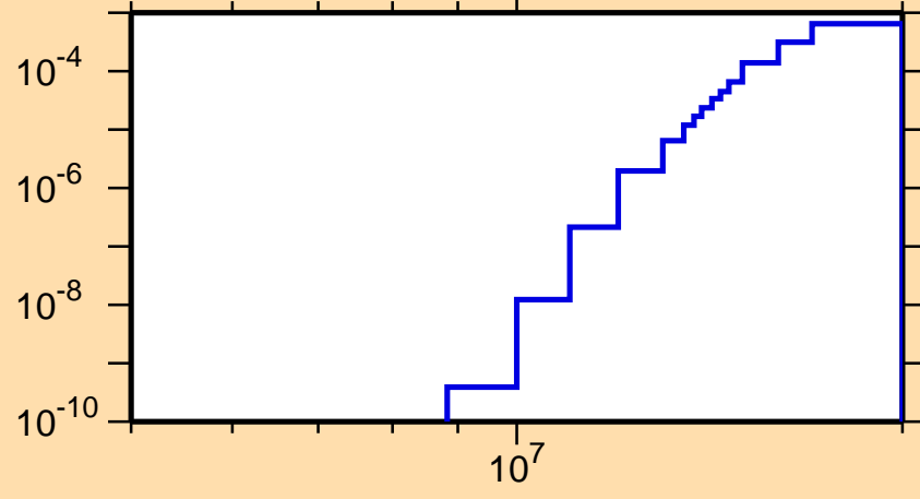
\sigma vs. E for ^{259}\text{No}(n,t)
