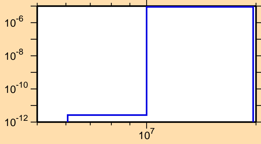
\sigma vs. E for ^{259}\text{No}(\text{mt } 45)
