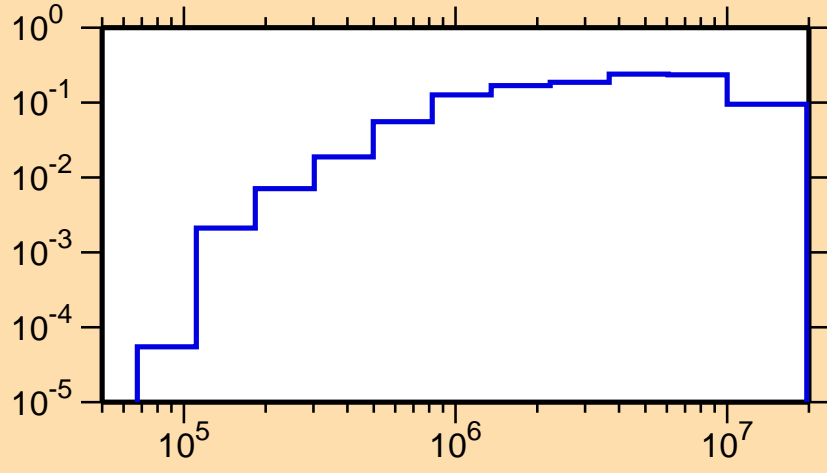
\sigma vs. E for ^{259}\text{No}(n,n\alpha)
