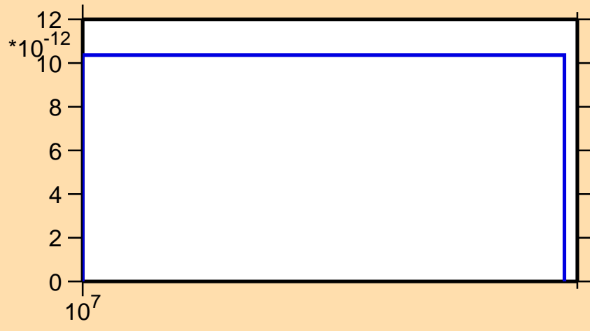
\sigma vs. E for ^{259}\text{No}(n,\text{He}3)
