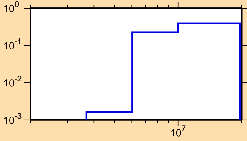
\sigma vs. E for ^{259}\text{No}(n,2n\alpha)
