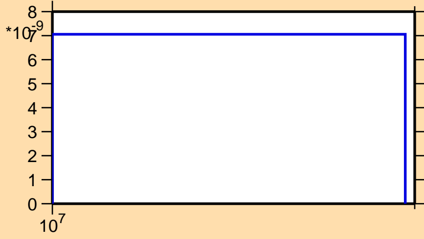
\sigma vs. E for ^{259}\text{No}(n,2np)
