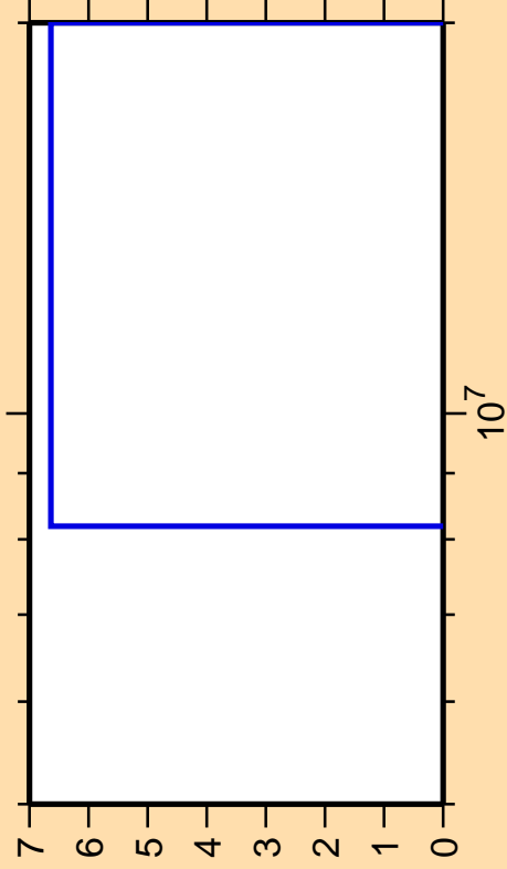
\Delta\sigma/\sigma vs. E for ^{259}\text{No}(n,\text{He}3)
