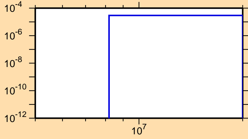
\sigma vs. E for ^{259}\text{No}(\text{mt117})
