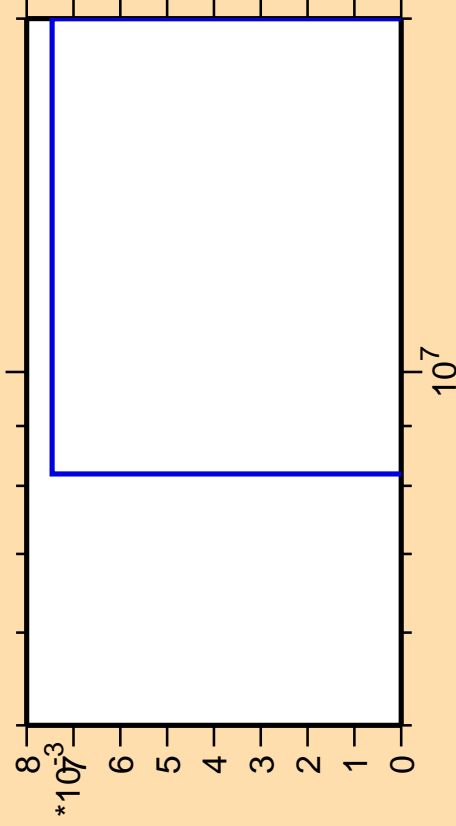
\Delta\sigma/\sigma vs. E for ^{259}\text{No}(\text{mt } 34)
