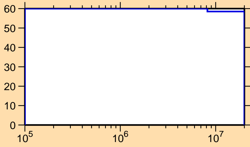
\Delta\sigma/\sigma vs. E for ^{259}\text{No}(n,n\text{cont.})
