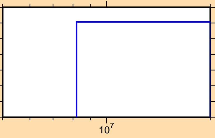
\sigma vs. E for ^{259}\text{No}(n,2np)
