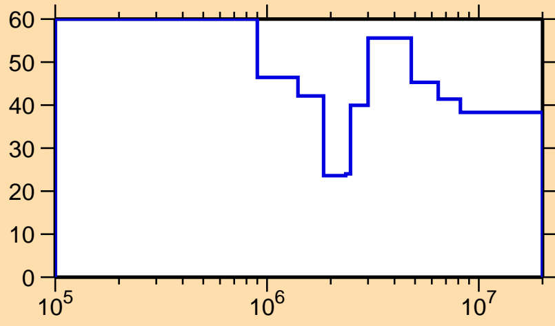
\Delta\sigma/\sigma vs. E for ^{259}\text{No}(n,n_1)
