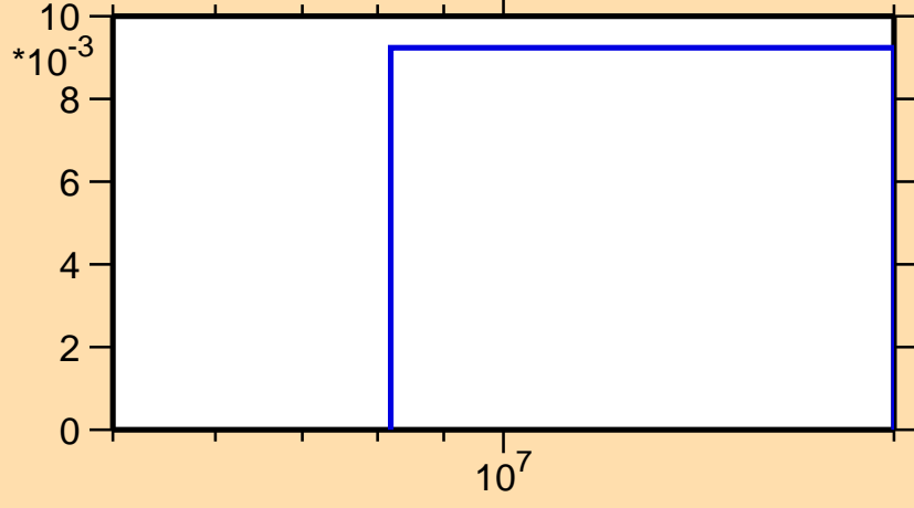
\sigma vs. E for ^{259}\text{No}(n,3n)
