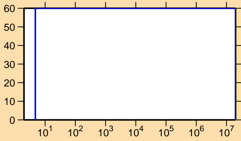
\Delta\sigma/\sigma vs. E for ^{259}\text{No}(n,\gamma)
