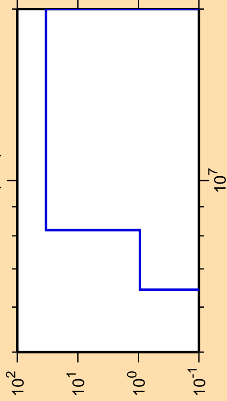
\Delta\sigma/\sigma vs. E for ^{259}\text{No}(n,d)
