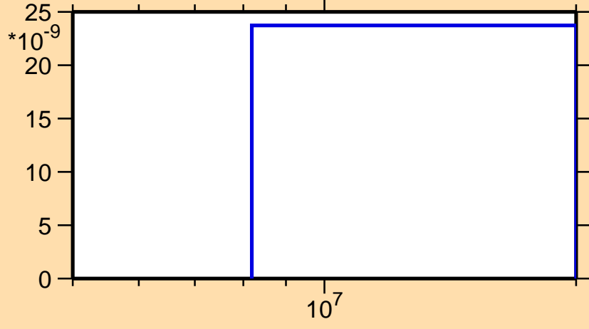
\sigma vs. E for ^{259}\text{No}(n,nt)
