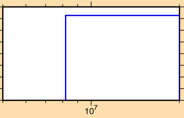
\sigma vs. E for ^{259}\text{No}(n,d)
