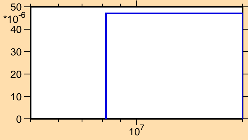
\sigma vs. E for ^{259}\text{No}(n,t)
