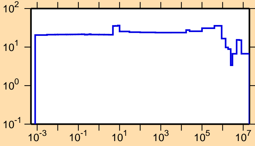
\Delta\sigma/\sigma vs. E for ^{259}\text{No}(n,el.)
