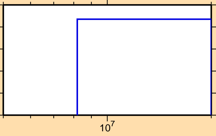
\sigma vs. E for ^{259}\text{No}(n,\text{He}3)
