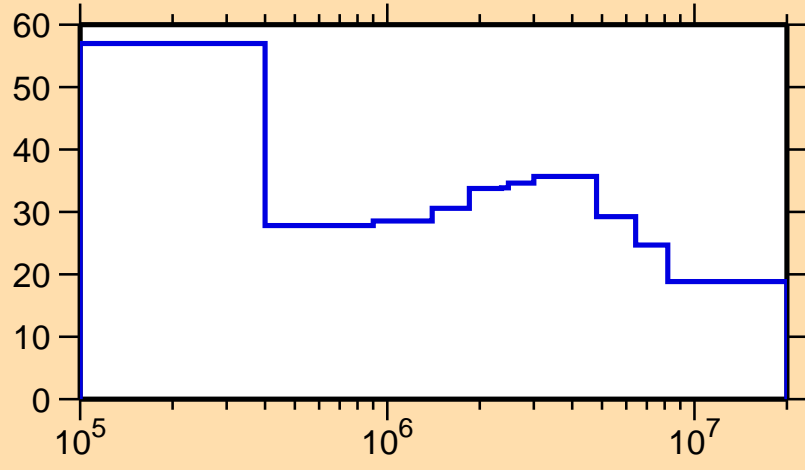
\Delta\sigma/\sigma vs. E for ^{259}\text{No}(n,f)
