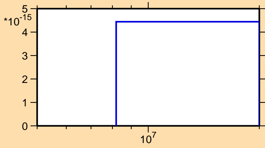
\sigma vs. E for ^{259}\text{No}(\text{mt } 34)
