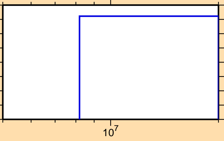
\sigma vs. E for ^{259}\text{No}(\text{mt } 45)
