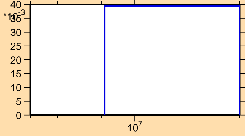
\sigma vs. E for ^{259}\text{No}(n,3n\alpha)
