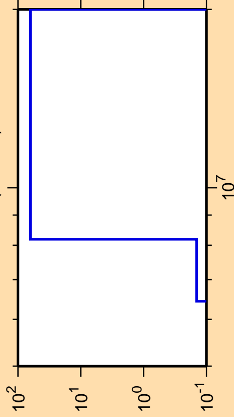
\Delta\sigma/\sigma vs. E for ^{259}\text{No}(\text{mt117})
