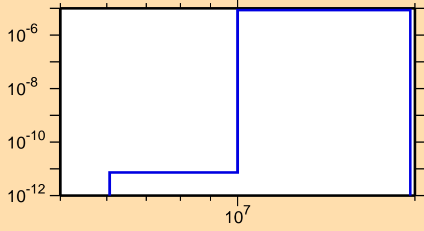
\sigma vs. E for ^{261}\text{No}(\text{mt117})
