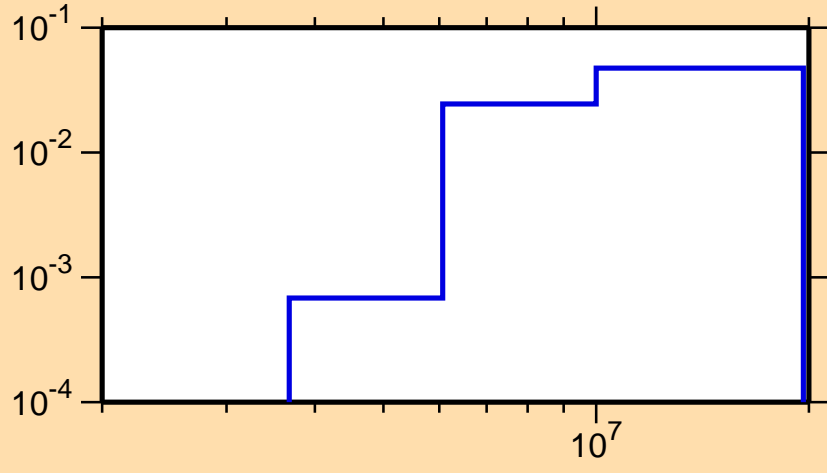
\sigma vs. E for ^{261}\text{No}(n,2n)
