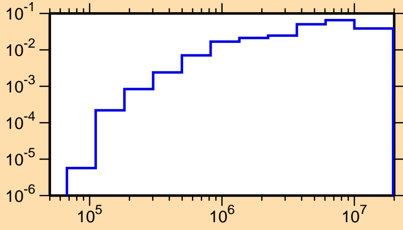
\sigma vs. E for ^{261}\text{No}(n,n\alpha)
