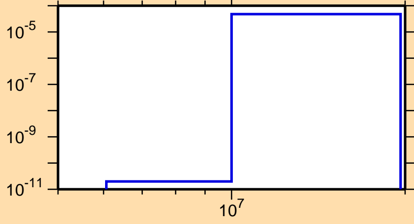
\sigma vs. E for ^{261}\text{No}(n,t)
