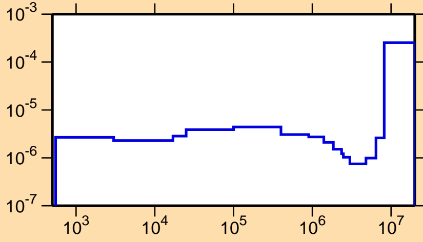
\sigma vs. E for ^{261}\text{No}(n,\alpha)
