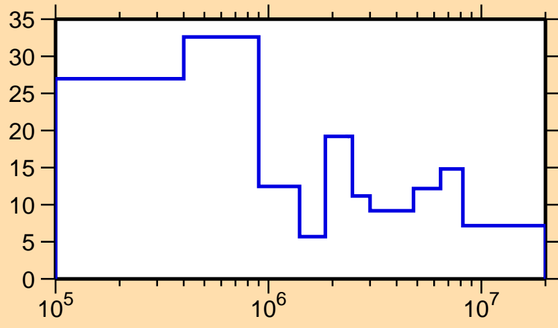
\Delta\sigma/\sigma vs. E for ^{261}\text{No}(n, el.)
