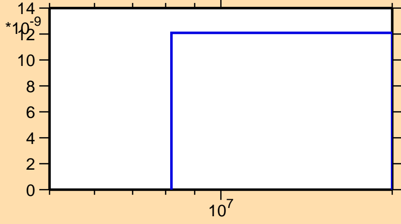
\sigma vs. E for ^{261}\text{No}(n,\text{nd})
