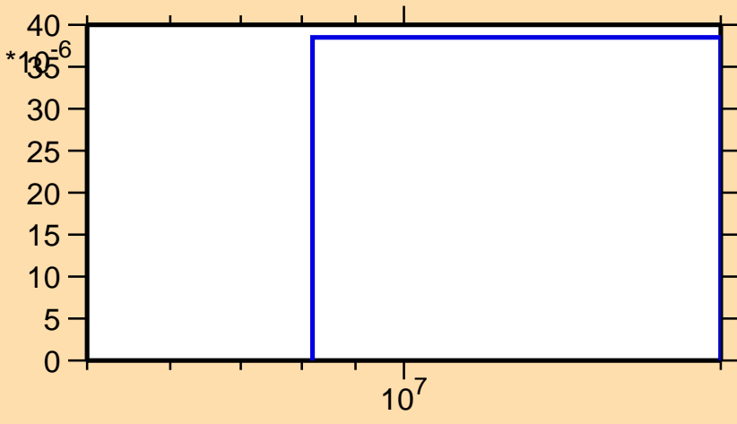
\sigma vs. E for ^{261}\text{No}(n,t)
