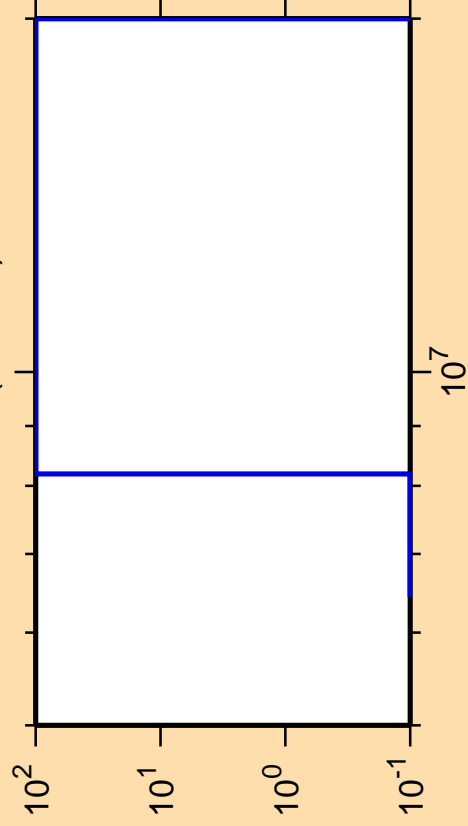
\Delta\sigma/\sigma vs. E for ^{261}\text{No}(\text{mt117})
