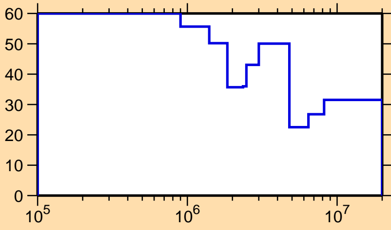
\Delta\sigma/\sigma vs. E for ^{261}\text{No}(n,n_1)
