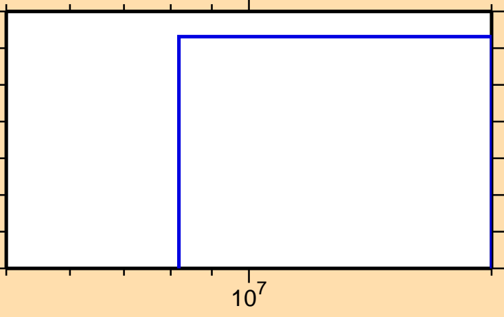
\sigma vs. E for ^{261}\text{No}(n,3n)
