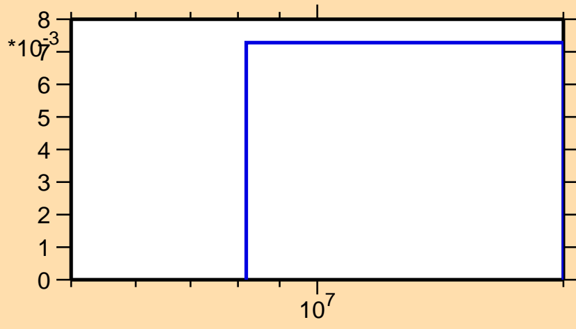
\sigma vs. E for ^{261}\text{No}(n,3n\alpha)
