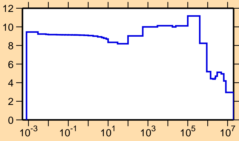
\sigma vs. E for ^{261}\text{No}(n,\text{el.})
