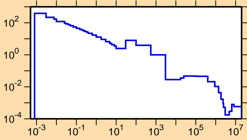
\sigma vs. E for ^{261}\text{No}(n,\gamma)
