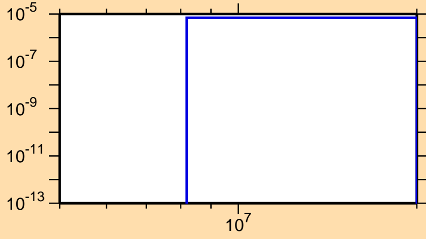
\sigma vs. E for ^{261}\text{No}(\text{mt117})
