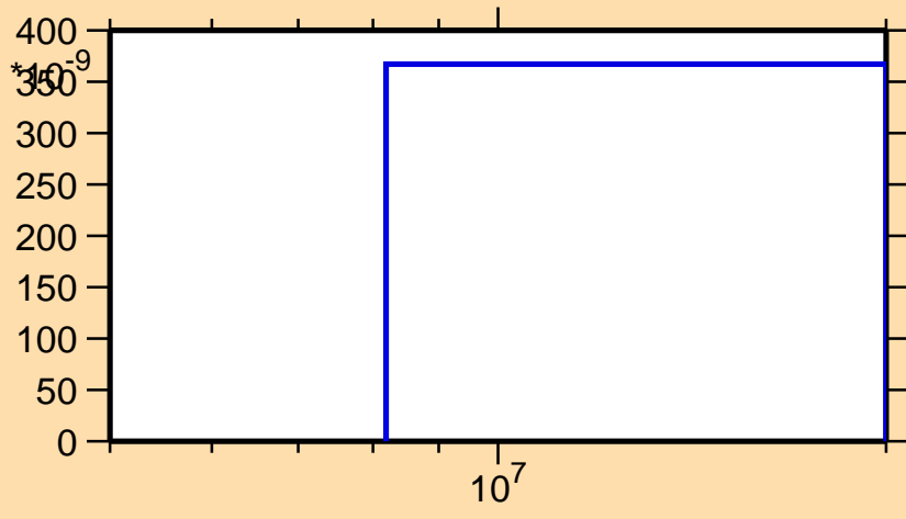
\sigma vs. E for ^{261}\text{No}(\text{mt } 45)
