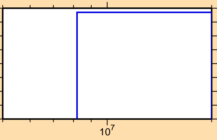
\sigma vs. E for ^{261}\text{No}(n,t)
