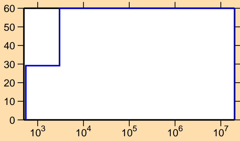
\Delta\sigma/\sigma vs. E for ^{261}\text{No}(n,\gamma)
