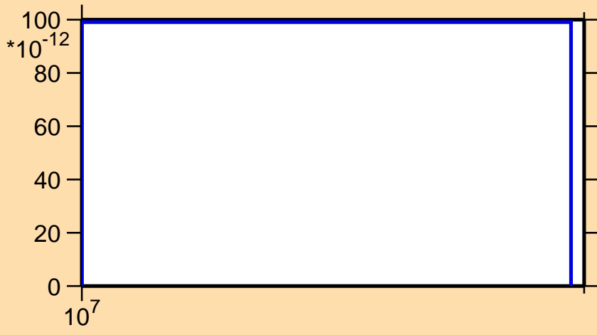
\sigma vs. E for ^{263}\text{No}(n,2np)
