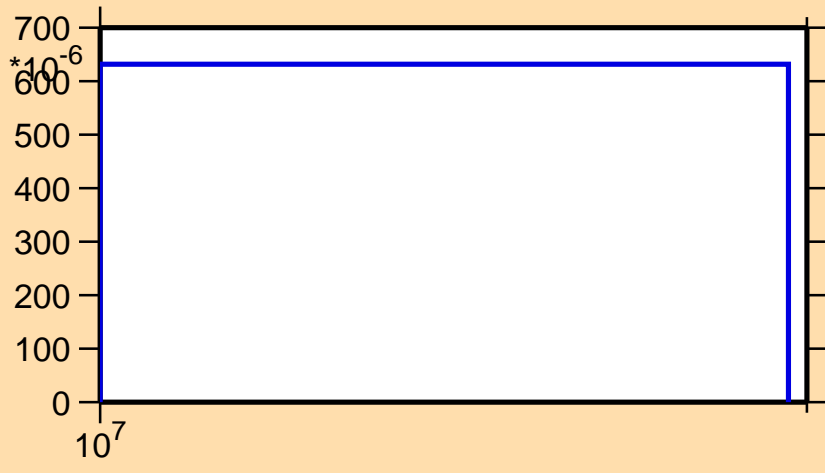
\sigma vs. E for ^{263}\text{No}(n,3n\alpha)
