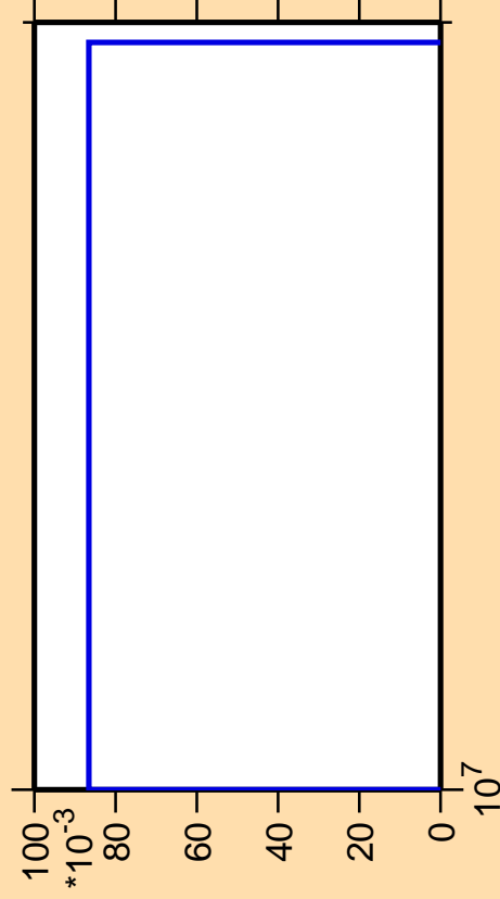
\Delta\sigma/\sigma vs. E for ^{263}\text{No}(\text{mt } 45)
