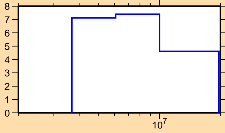
\Delta\sigma/\sigma vs. E for ^{263}\text{No}(n,f)
