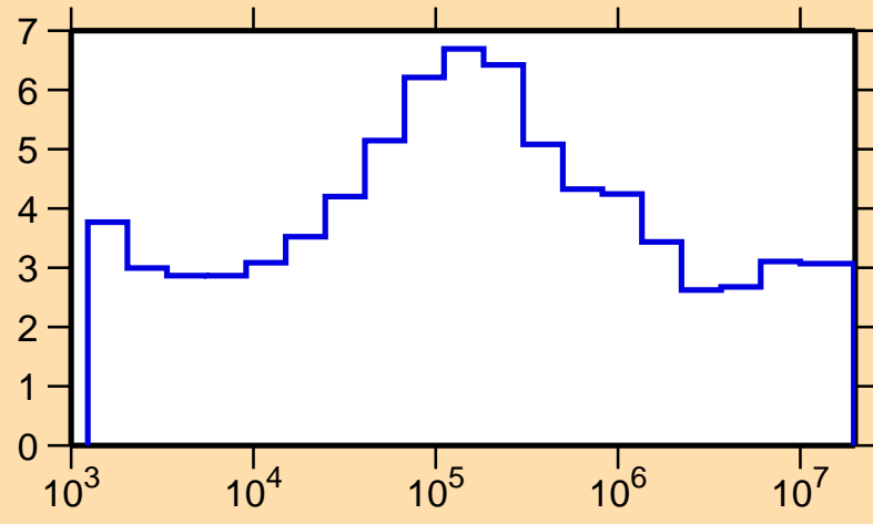
\sigma vs. E for ^{263}\text{No}(n,\text{nonel.})
