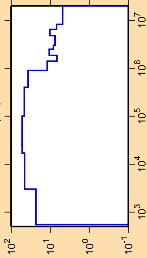
\Delta\sigma/\sigma vs. E for ^{263}\text{No}(n,f)
