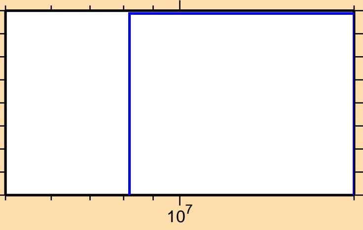
\sigma vs. E for ^{263}\text{No}(n,\text{nd})
