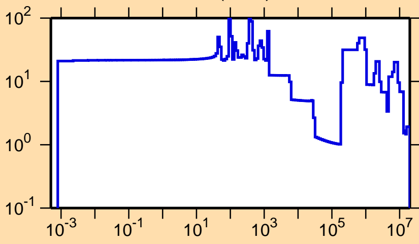
\Delta\sigma/\sigma vs. E for ^{264}\text{No}(n,el.)
