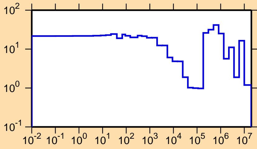
\Delta\sigma/\sigma vs. E for ^{264}\text{No}(n,el.)
