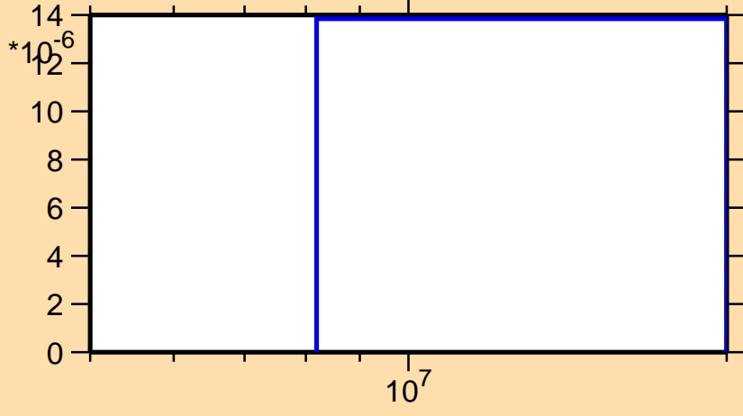
\sigma vs. E for ^{264}\text{No}(n,d)
