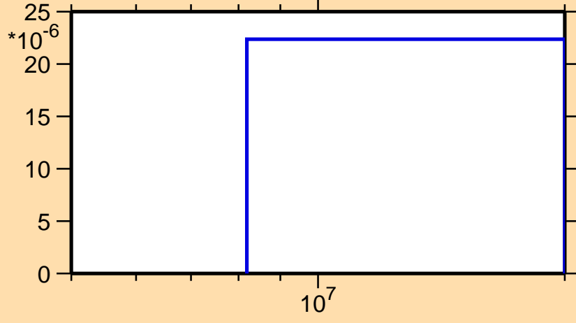
\sigma vs. E for ^{264}\text{No}(n,t)
