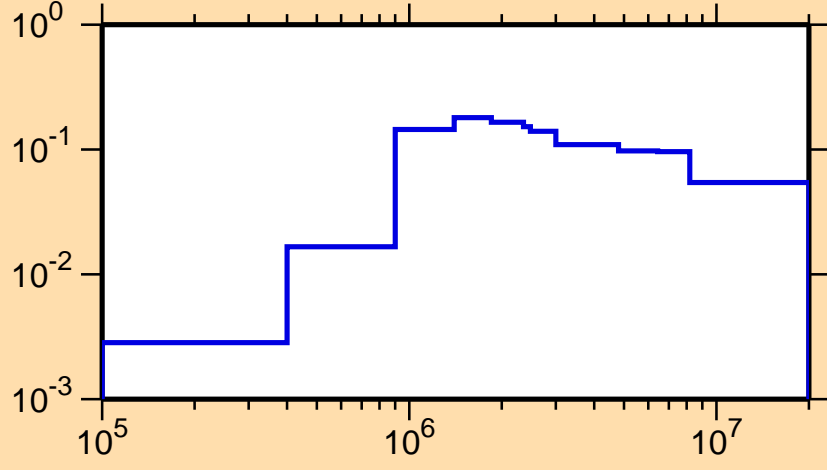
\sigma vs. E for ^{264}\text{No}(n,n\text{cont.})
