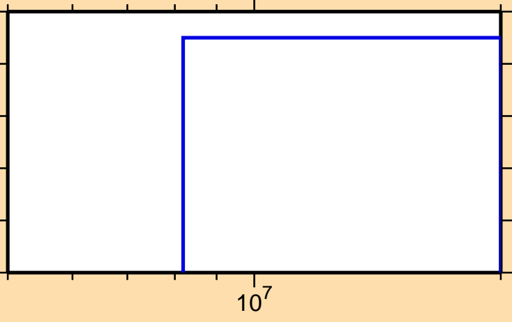
\sigma vs. E for ^{264}\text{No}(n,\text{He3})
