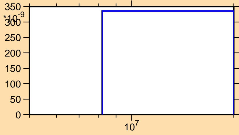
\sigma vs. E for ^{264}\text{No}(n,np)
