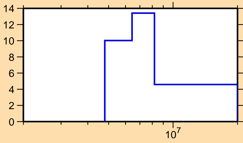
\Delta\sigma/\sigma vs. E for ^{264}\text{No}(n,\text{tot.})
