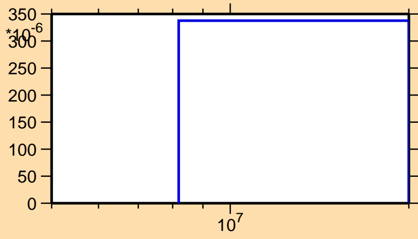
\sigma vs. E for ^{264}\text{No}(n,3n\alpha)
