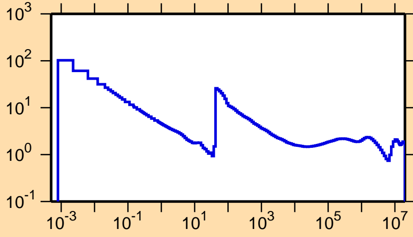
\sigma vs. E for ^{228}\text{Np}(n,f)
