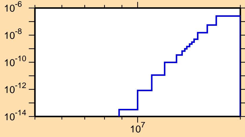
\sigma vs. E for ^{228}\text{Np}(n,\text{He3})
