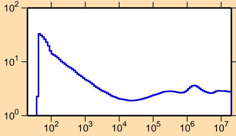
\sigma vs. E for ^{228}\text{Np}(n,\text{nonel.})
