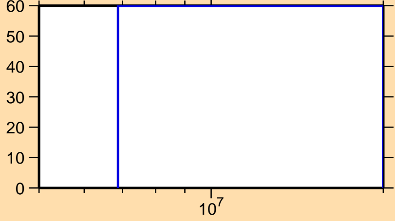
\Delta\sigma/\sigma vs. E for ^{228}\text{Np}(n,2n)
