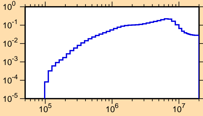
\sigma vs. E for ^{228}\text{Np}(n,n\alpha)
