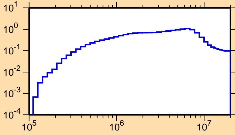
\sigma vs. E for ^{228}\text{Np}(n,n\text{cont.})
