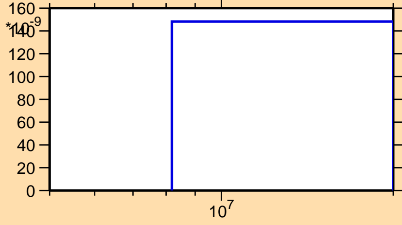
\sigma vs. E for ^{228}\text{Np}(n,\text{nd})
