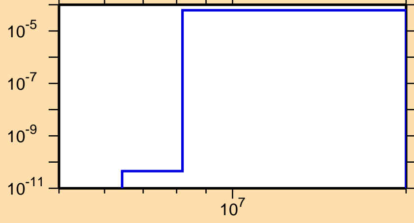
\sigma vs. E for ^{228}\text{Np}(n,t)
