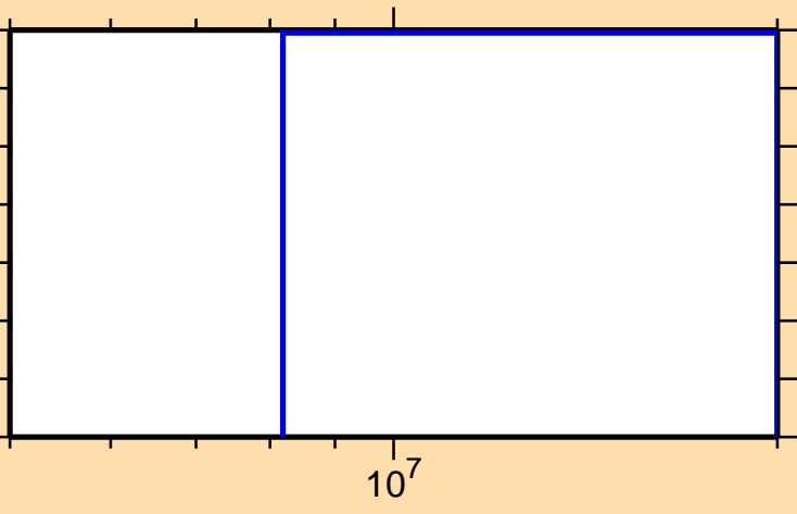
\sigma vs. E for ^{228}\text{Np}(n,\text{He3})
