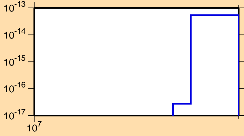
\sigma vs. E for ^{229}\text{Np} (mt 11)
