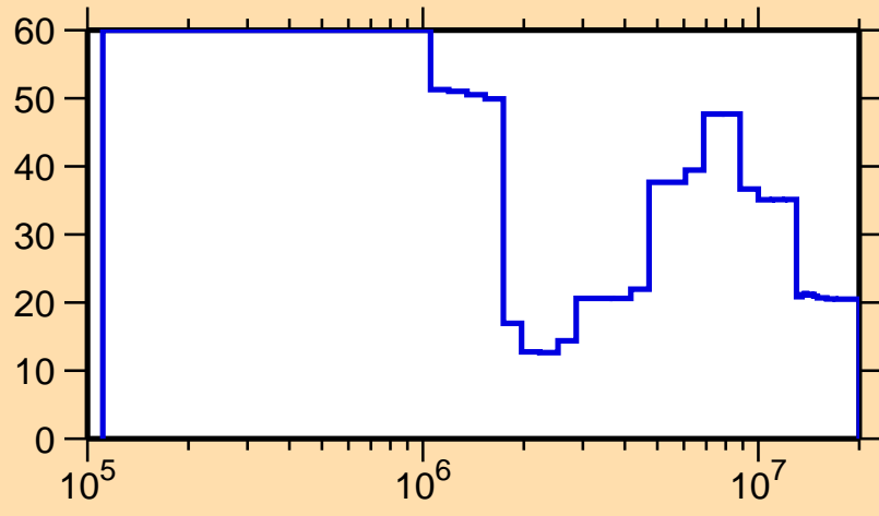
\Delta\sigma/\sigma vs. E for ^{229}\text{Np}(n,\text{el.})
