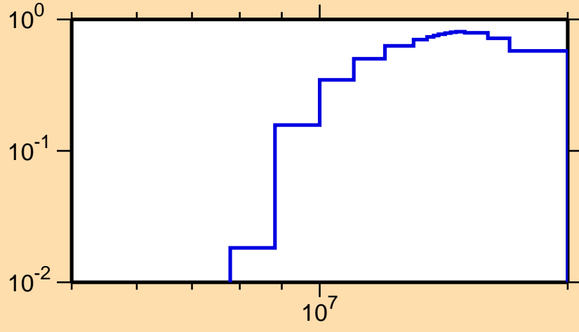
\sigma vs. E for ^{229}\text{Np}(n,2n)
