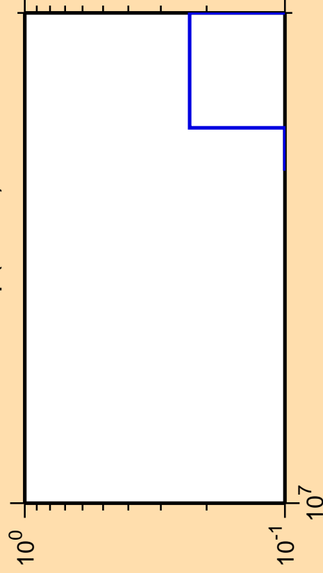
\Delta\sigma/\sigma vs. E for ^{229}\text{Np} (mt 11)
