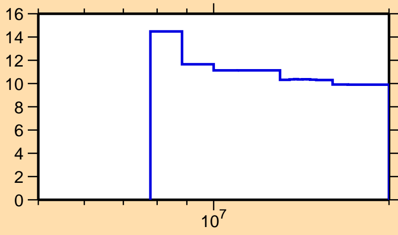
\Delta\sigma/\sigma vs. E for ^{229}\text{Np}(n,\text{nonel.})
