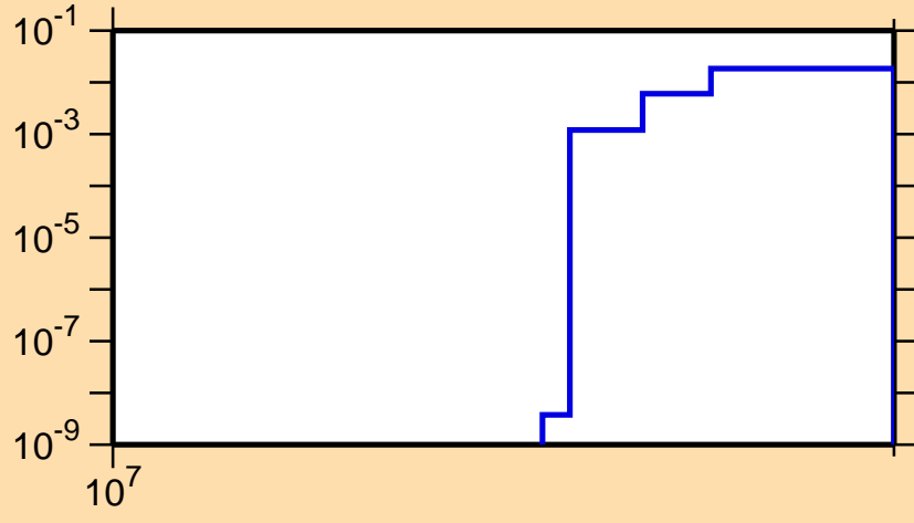
\sigma vs. E for ^{229}\text{Np}(n,3n)
