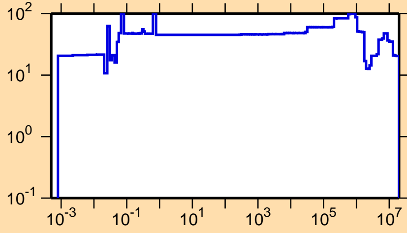
\Delta\sigma/\sigma vs. E for ^{229}\text{Np}(n,el.)
