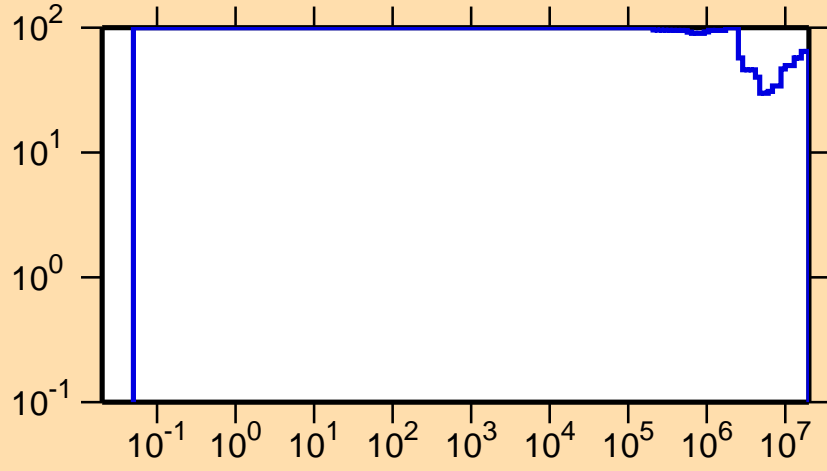
\Delta\sigma/\sigma vs. E for ^{229}\text{Np}(n,p)
