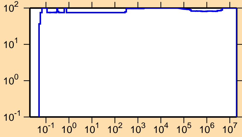
\Delta\sigma/\sigma vs. E for ^{229}\text{Np}(n,\gamma)
