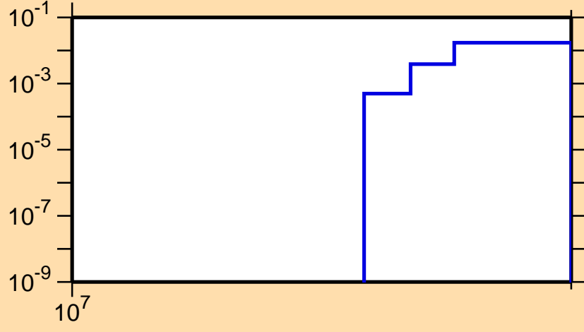
\sigma vs. E for ^{229}\text{Np}(n,3n\alpha)
