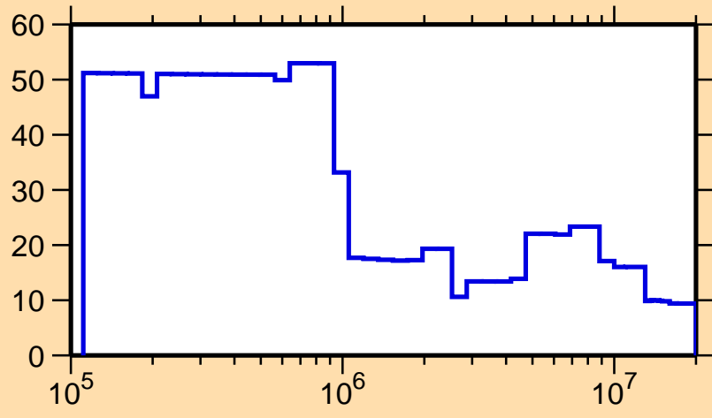
\Delta\sigma/\sigma vs. E for ^{229}\text{Np}(n,\text{tot.})
