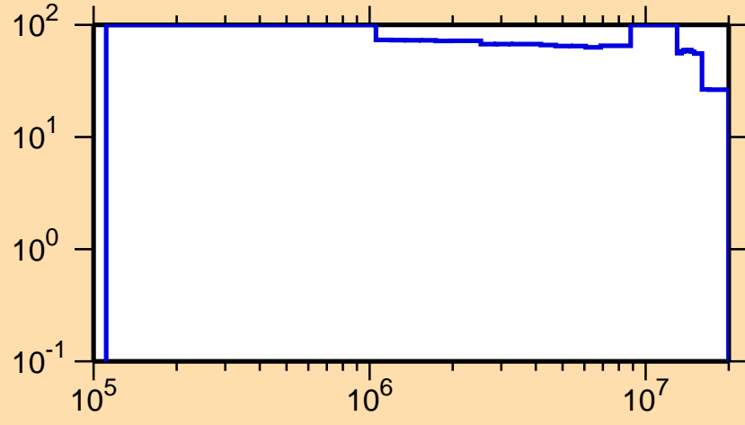
\Delta\sigma/\sigma vs. E for ^{229}\text{Np}(n,n\text{cont.})
