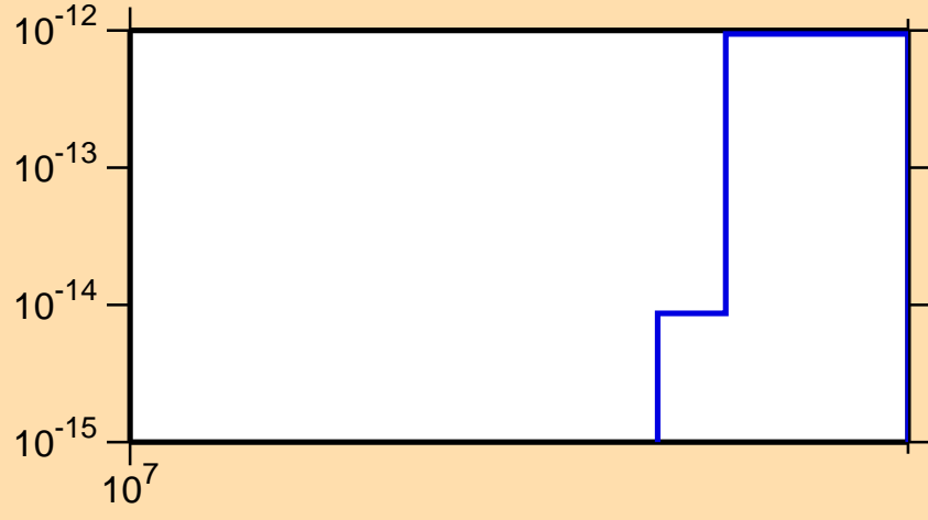
\sigma vs. E for ^{229}\text{Np} (mt 34)
