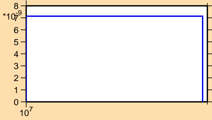
\sigma vs. E for ^{229}\text{Np}(n,nt)
