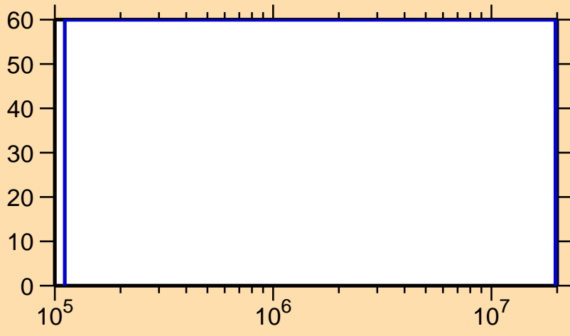
\Delta\sigma/\sigma vs. E for ^{229}\text{Np}(n,n_1)
