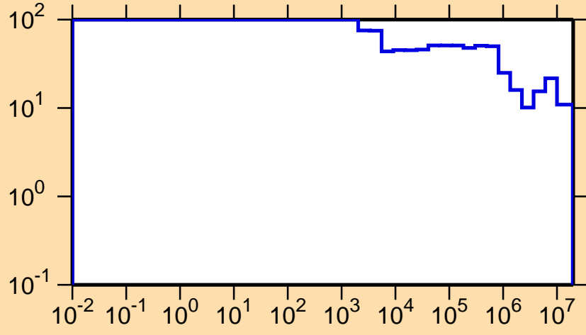
\Delta\sigma/\sigma vs. E for ^{229}\text{Np}(n,tot.)
