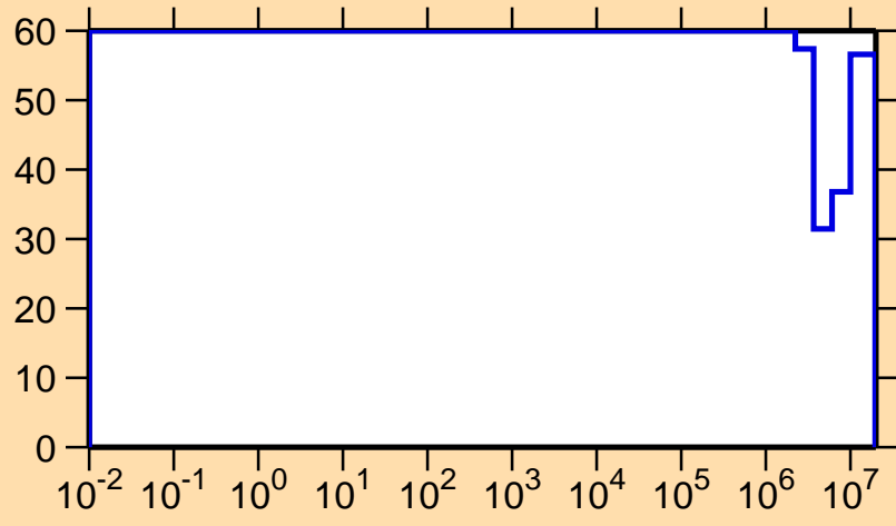
\Delta\sigma/\sigma vs. E for ^{229}\text{Np}(n,p)
