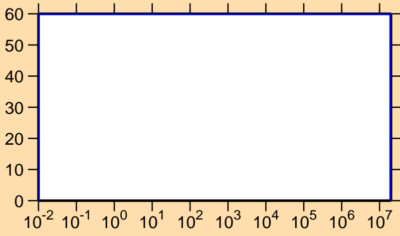
\Delta\sigma/\sigma vs. E for ^{229}\text{Np}(n,\gamma)
