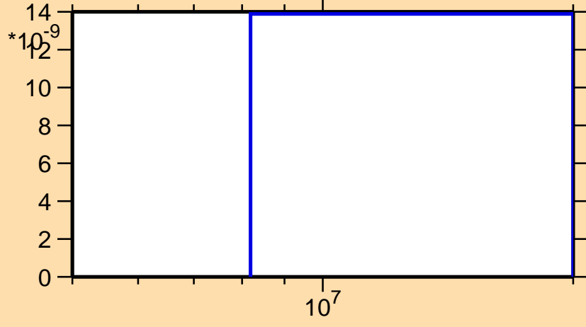
\sigma vs. E for ^{229}\text{Np}(n,nd)
