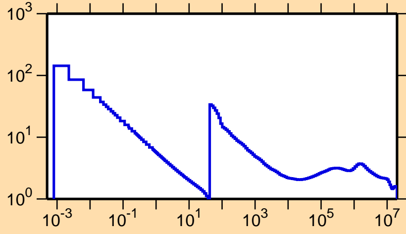
\sigma vs. E for ^{230}\text{Np}(n,f)
