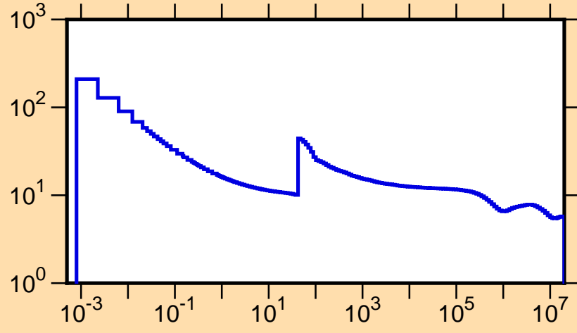
\sigma vs. E for ^{230}\text{Np}(n,\text{tot.})
