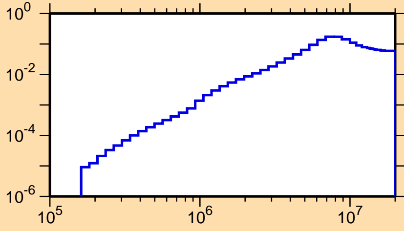
\sigma vs. E for ^{230}\text{Np}(n,n\alpha)
