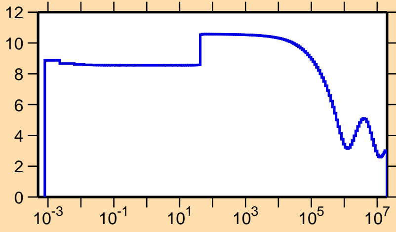
\sigma vs. E for ^{230}\text{Np}(n,\text{el.})
