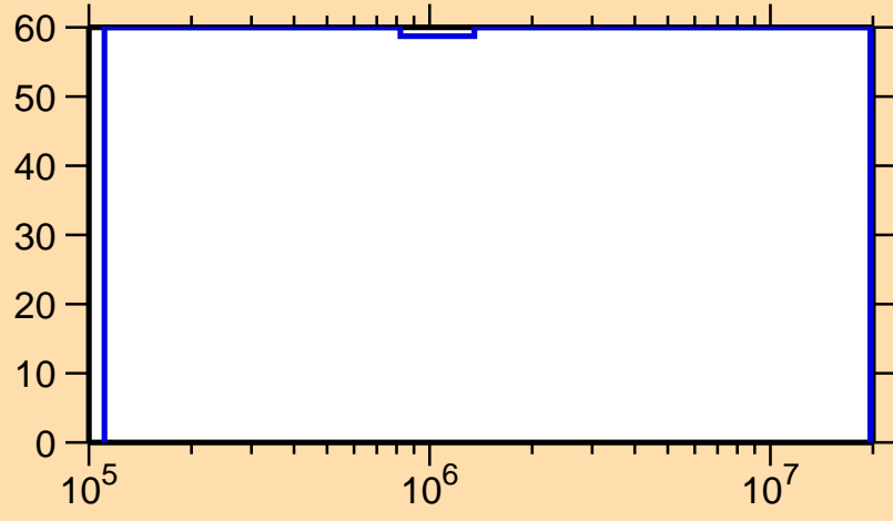
\Delta\sigma/\sigma vs. E for ^{230}\text{Np}(n,n\text{cont.})
