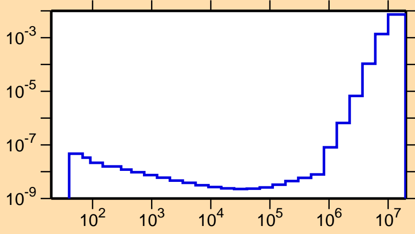
\sigma vs. E for ^{230}\text{Np}(n,p)
