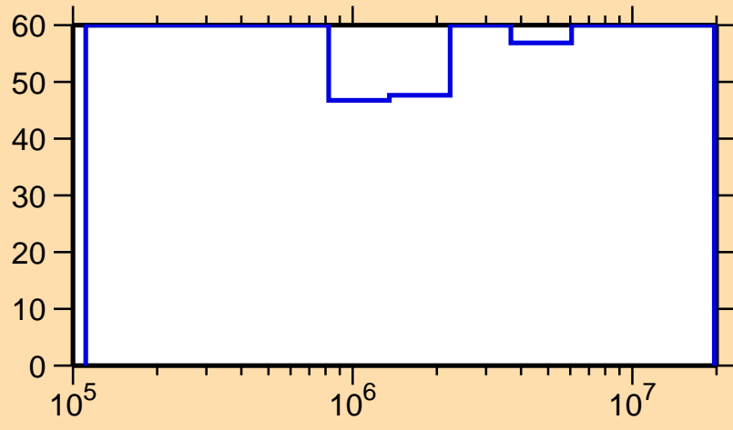
\Delta\sigma/\sigma vs. E for ^{230}\text{Np}(n,\text{inel.})
