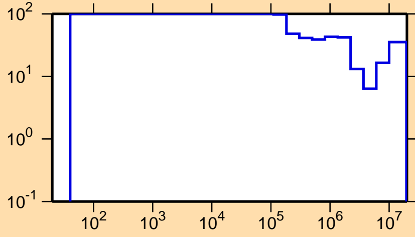
\Delta\sigma/\sigma vs. E for ^{230}\text{Np}(n,f)
