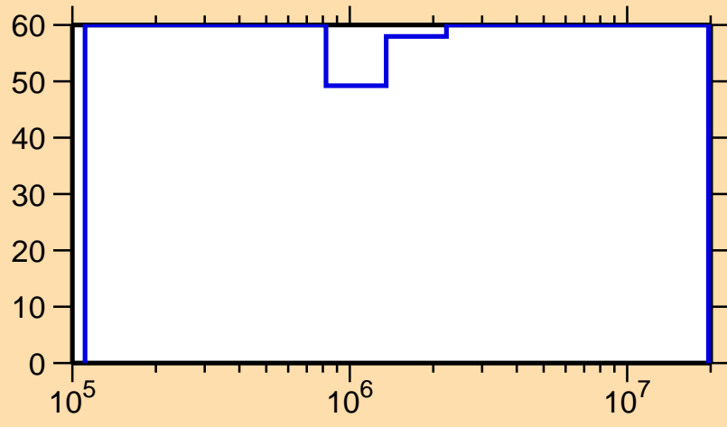
\Delta\sigma/\sigma vs. E for ^{230}\text{Np}(n,n_1)
