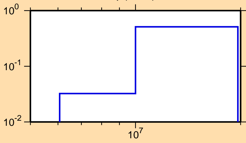
\sigma vs. E for ^{230}\text{Np}(n,2n)
