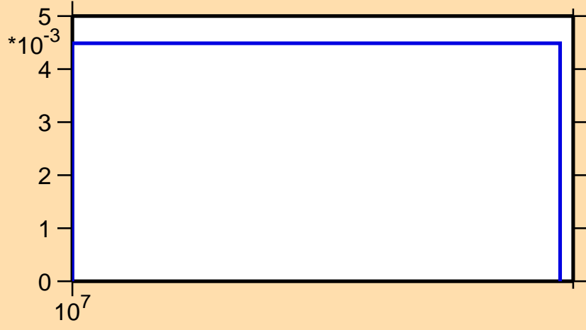
\sigma vs. E for ^{230}\text{Np}(n,3n)
