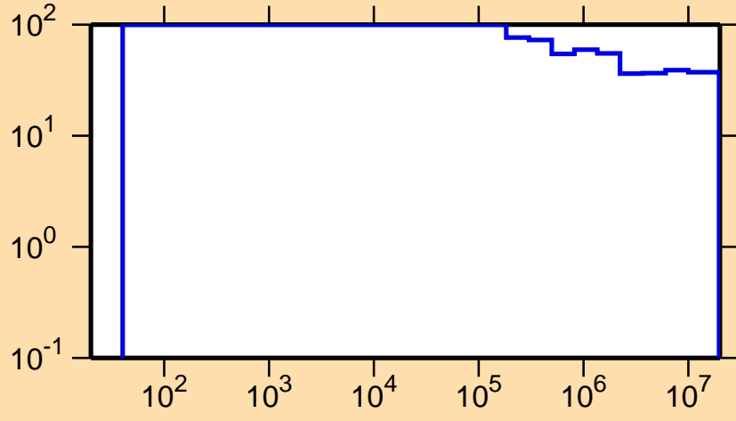
\Delta\sigma/\sigma vs. E for ^{230}\text{Np}(n,p)
