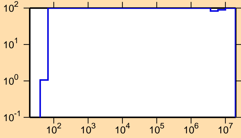
\Delta\sigma/\sigma vs. E for ^{230}\text{Np}(n,\gamma)
