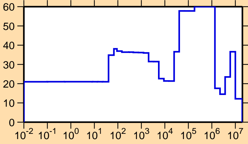
\Delta\sigma/\sigma vs. E for ^{230}\text{Np}(n,el.)
