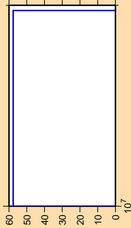
\Delta\sigma/\sigma vs. E for ^{230}\text{Np}(n,3n\alpha)
