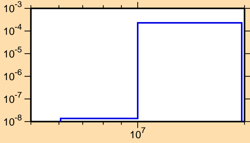
\sigma vs. E for ^{230}\text{Np}(\text{mt117})
