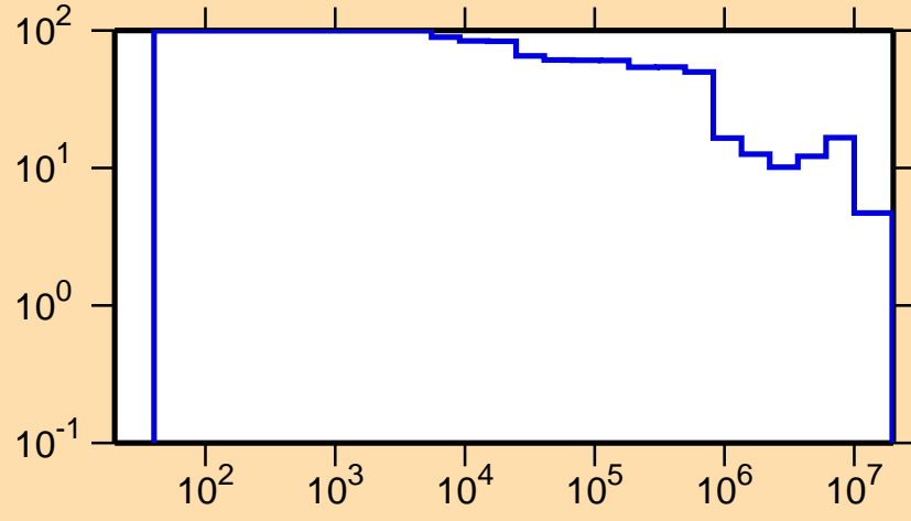
\Delta\sigma/\sigma vs. E for ^{230}\text{Np}(n,\text{tot.})
