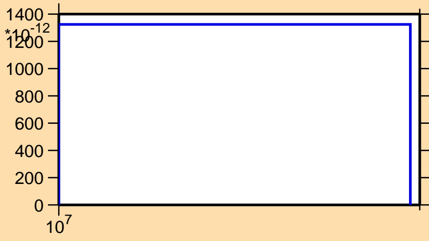
\sigma vs. E for ^{230}\text{Np}(n,\text{He}3)
