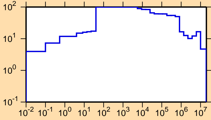
\Delta\sigma/\sigma vs. E for ^{230}\text{Np}(n,tot.)
