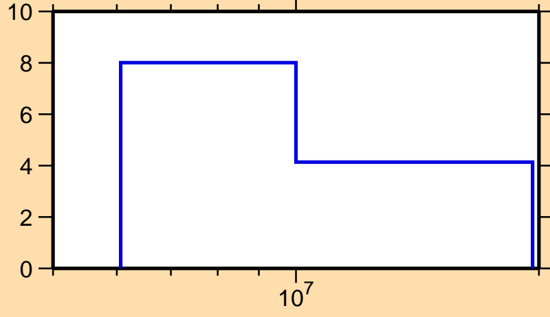
\Delta\sigma/\sigma vs. E for ^{230}\text{Np}(n,\text{nonel.})
