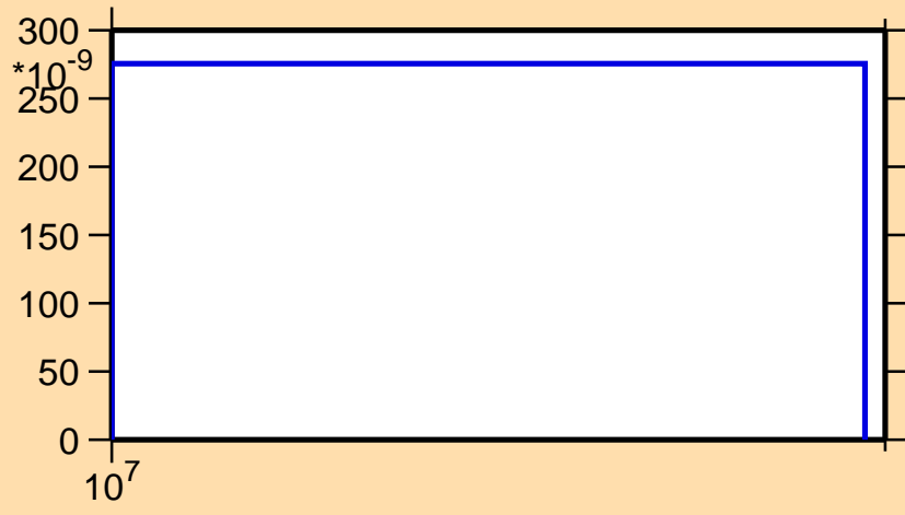
\sigma vs. E for ^{230}\text{Np}(n,2np)
