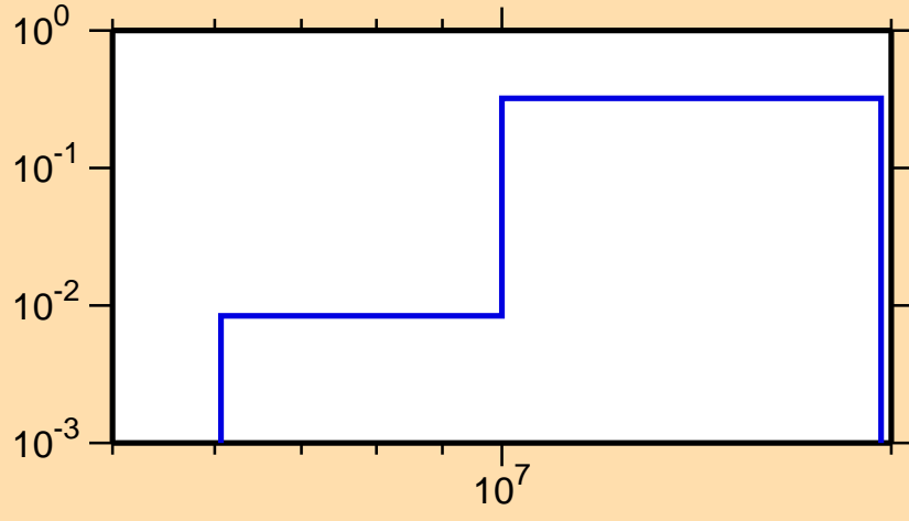
\sigma vs. E for ^{230}\text{Np}(n,2n\alpha)
