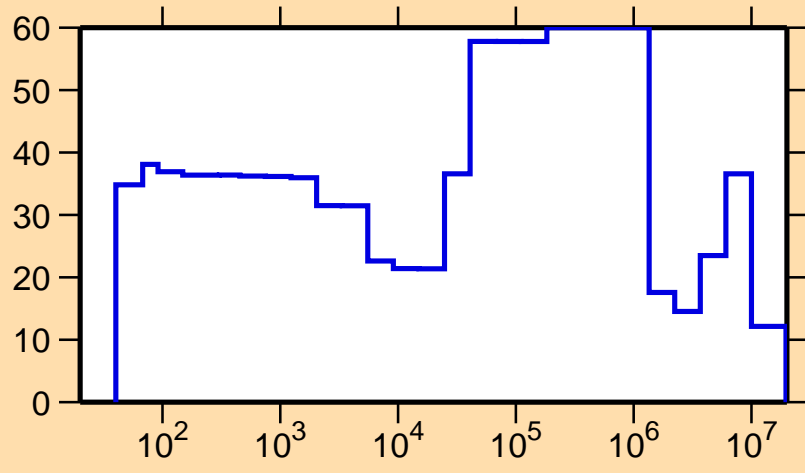
\Delta\sigma/\sigma vs. E for ^{230}\text{Np}(n,el.)
