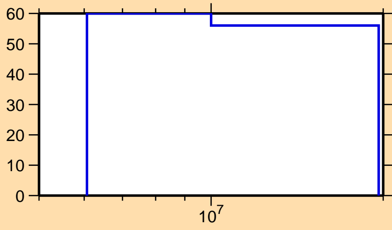
\Delta\sigma/\sigma vs. E for ^{230}\text{Np}(n,2n)
