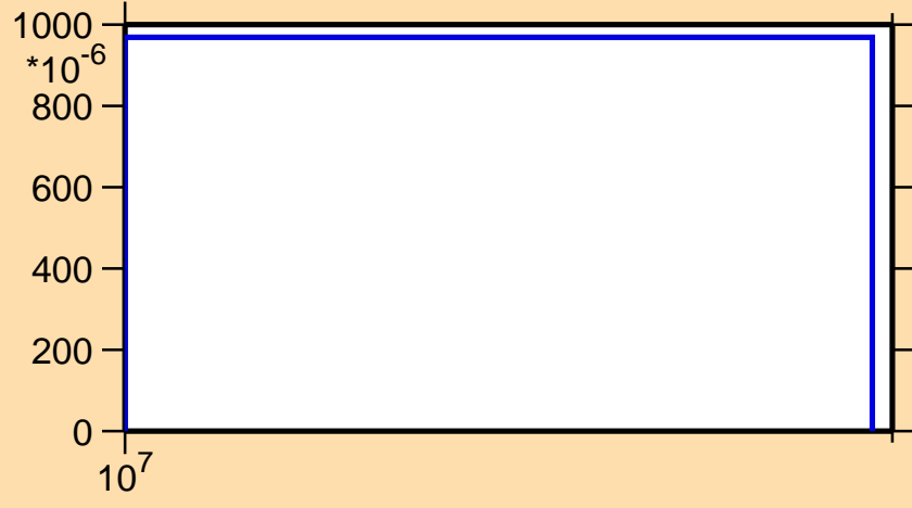
\sigma vs. E for ^{230}\text{Np}(n,3n\alpha)
