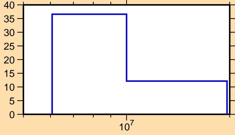
\Delta\sigma/\sigma vs. E for ^{230}\text{Np}(n,\text{el.})
