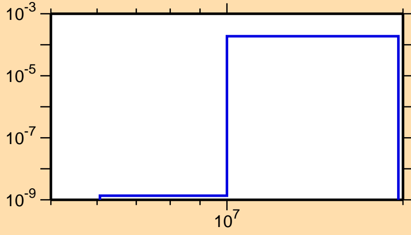
\sigma vs. E for ^{230}\text{Np}(n,t)
