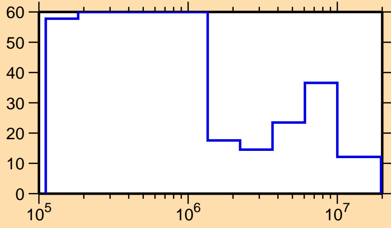
\Delta\sigma/\sigma vs. E for ^{230}\text{Np}(n,\text{el.})
