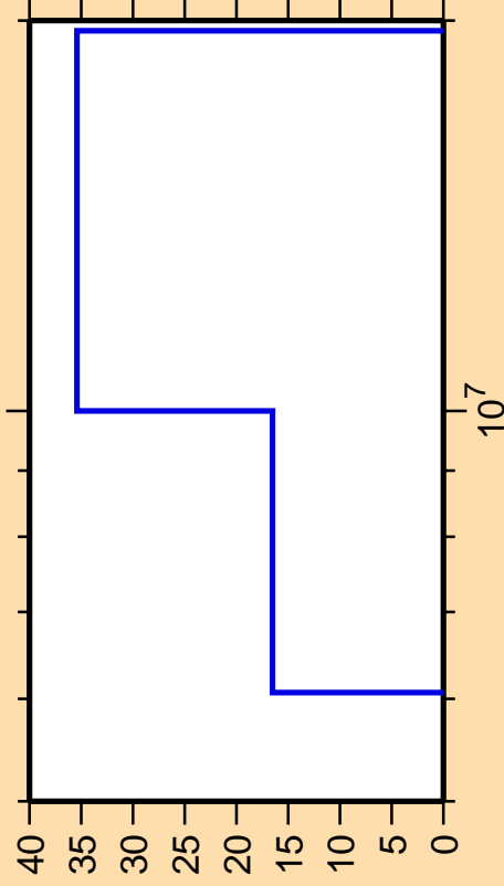
\Delta\sigma/\sigma vs. E for ^{230}\text{Np}(n,f)
