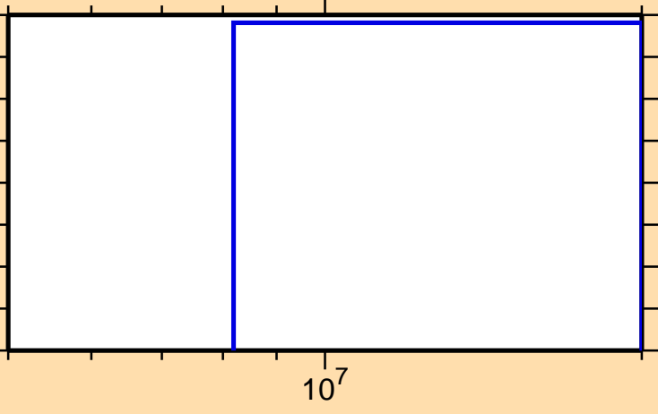
\sigma vs. E for ^{230}\text{Np}(n,3n\alpha)
