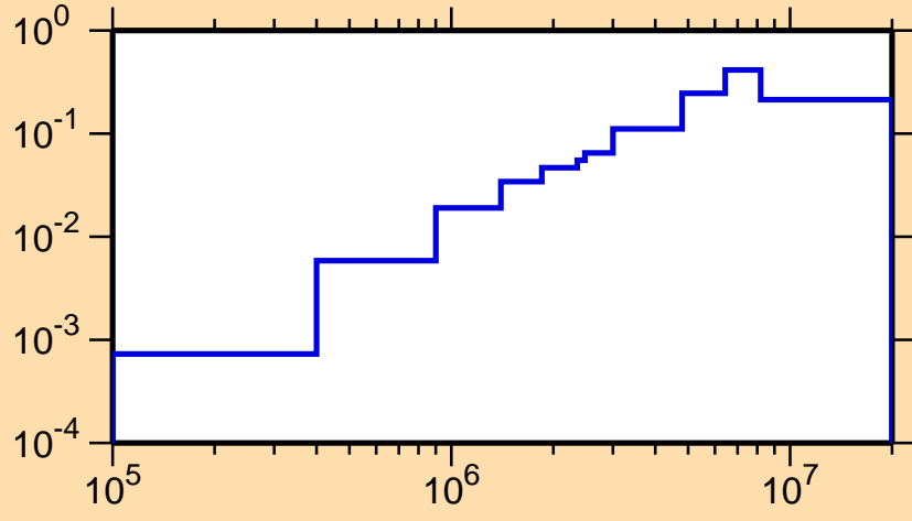
\sigma vs. E for ^{230}\text{Np}(n,\text{inel.})
