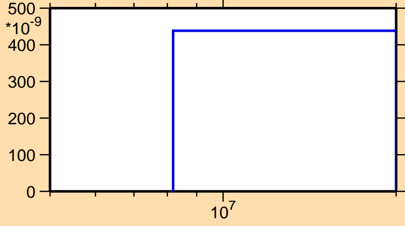
\sigma vs. E for ^{230}\text{Np}(n,\text{nd})
