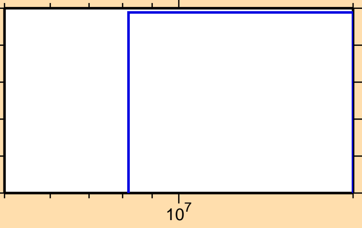
\sigma vs. E for ^{230}\text{Np}(n,nt)
