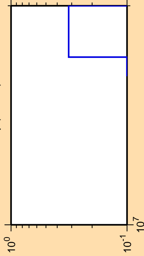
\Delta\sigma/\sigma vs. E for ^{231}\text{Np} (mt 11)
