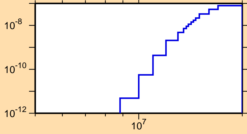
\sigma vs. E for ^{231}\text{Np}(\text{mt117})
