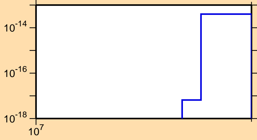
\sigma vs. E for ^{231}\text{Np} (mt 11)
