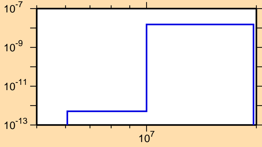
\sigma vs. E for ^{231}\text{Np}(\text{mt117})
