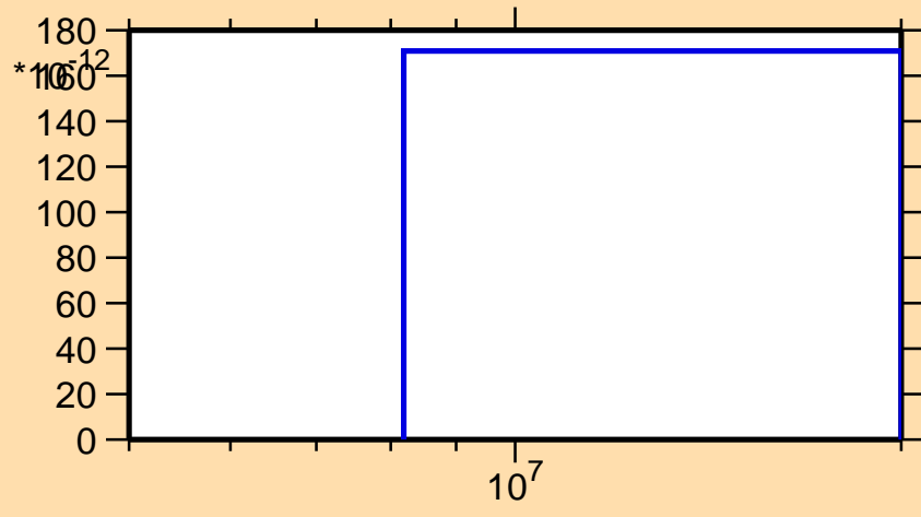
\sigma vs. E for ^{231}\text{Np}(n,nd)
