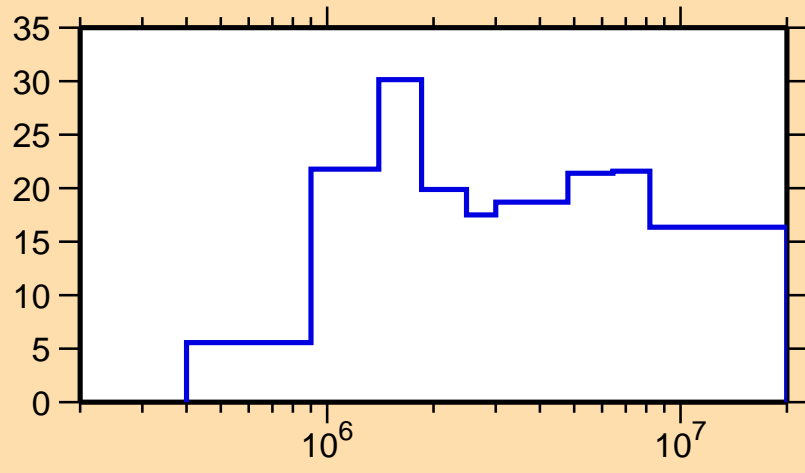
\Delta\sigma/\sigma vs. E for ^{231}\text{Np}(n,p)
