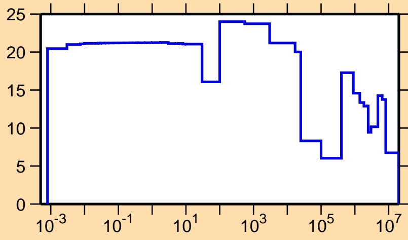
\Delta\sigma/\sigma vs. E for ^{231}\text{Np}(n,el.)
