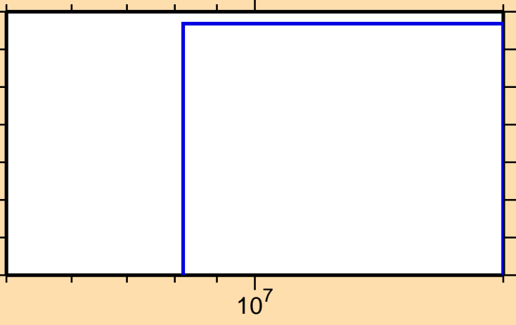
\sigma vs. E for ^{231}\text{Np} (mt 45)
