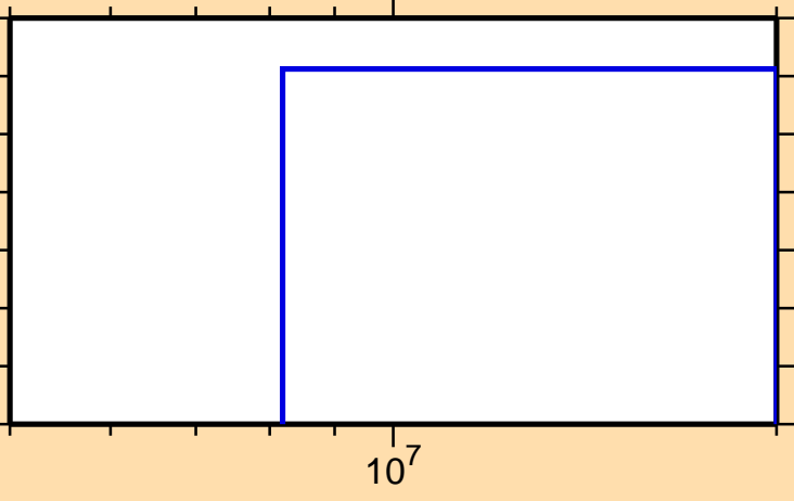
\sigma vs. E for ^{231}\text{Np}(\text{mt117})
