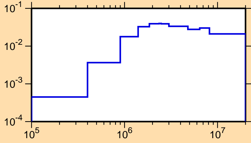
\sigma vs. E for ^{231}\text{Np}(n,n\text{cont.})
