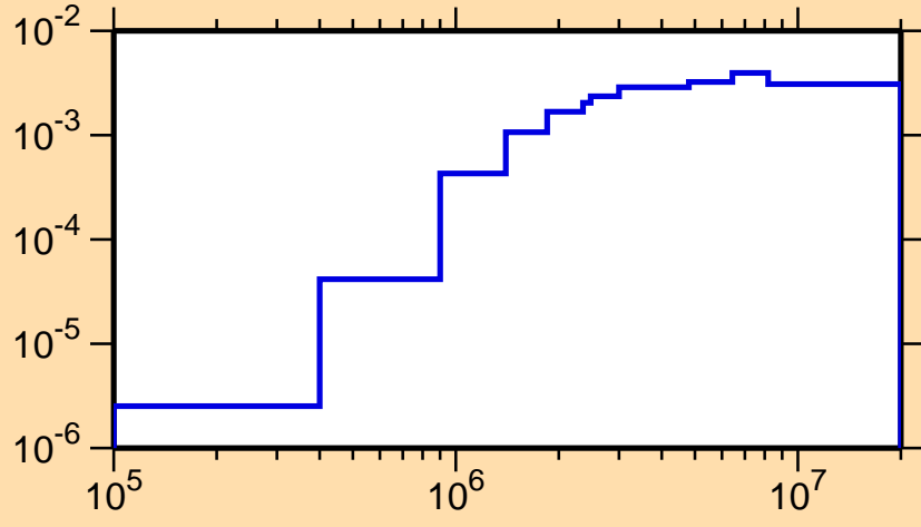
\sigma vs. E for ^{231}\text{Np}(n,n\alpha)
