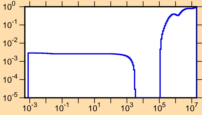
\mu vs. E for ^{232}\text{Np}(\text{mt251})
