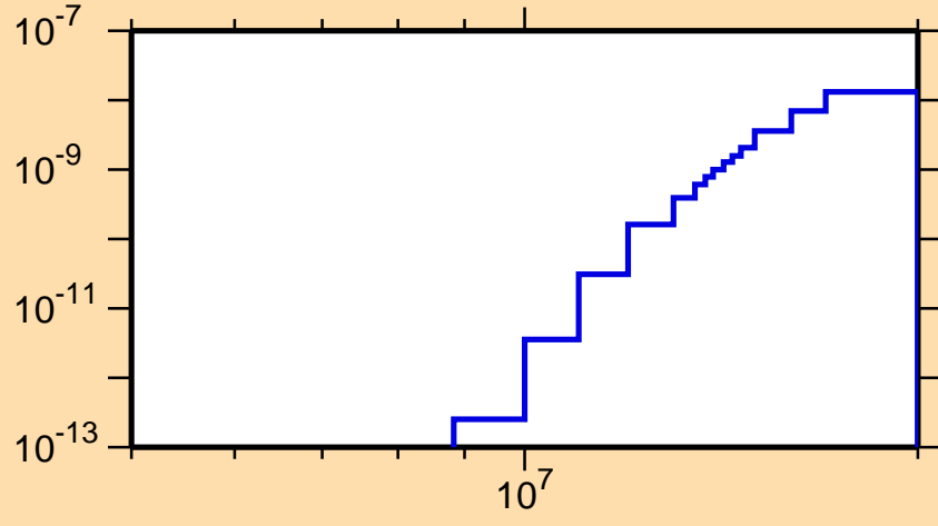
\sigma vs. E for ^{232}\text{Np}(\text{mt117})
