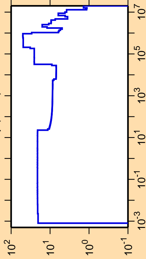
\Delta\sigma/\sigma vs. E for ^{232}\text{Np}(n,\text{el.})
