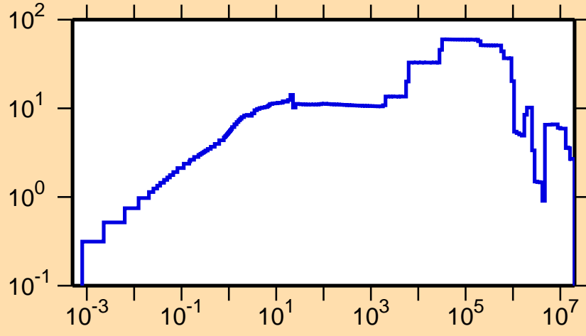
\Delta\sigma/\sigma vs. E for ^{232}\text{Np}(n,tot.)
