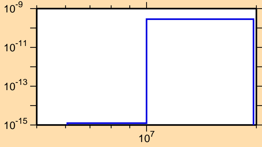
\sigma vs. E for ^{232}\text{Np} (mt 45)
