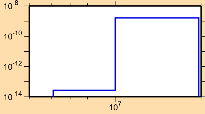
\sigma vs. E for ^{232}\text{Np}(\text{mt117})
