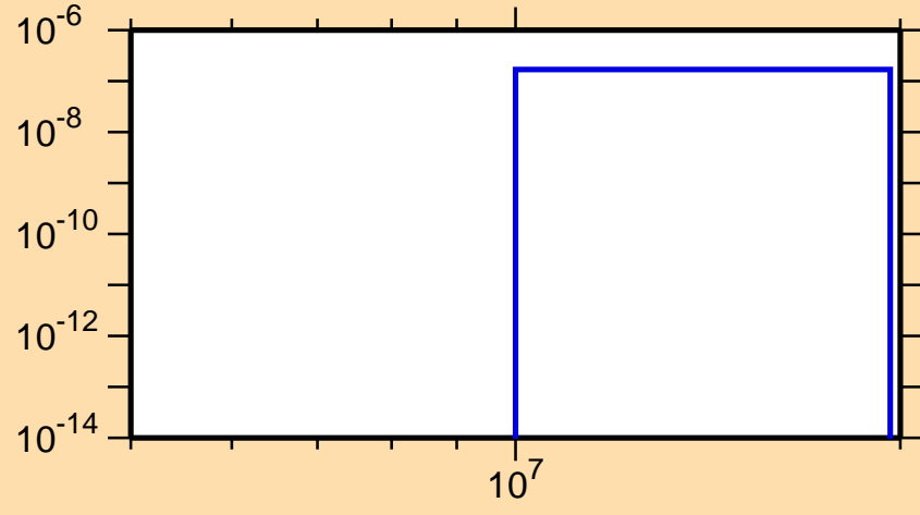
\sigma vs. E for ^{232}\text{Np}(n,\text{nd})
