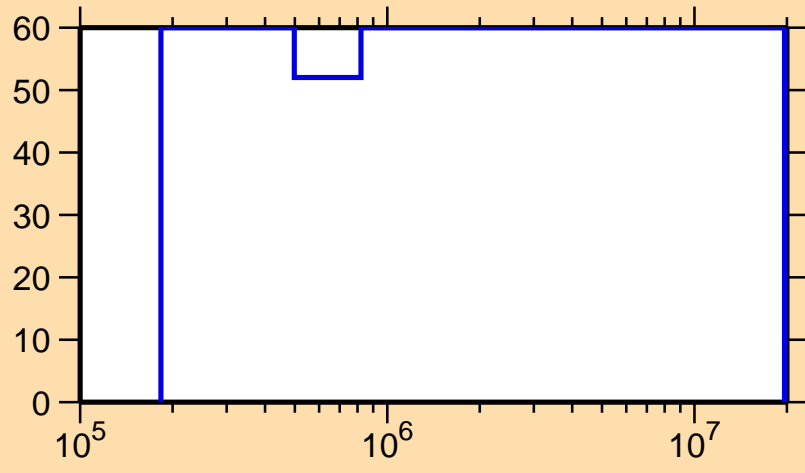
\Delta\sigma/\sigma vs. E for ^{232}\text{Np}(n,n\text{cont.})
