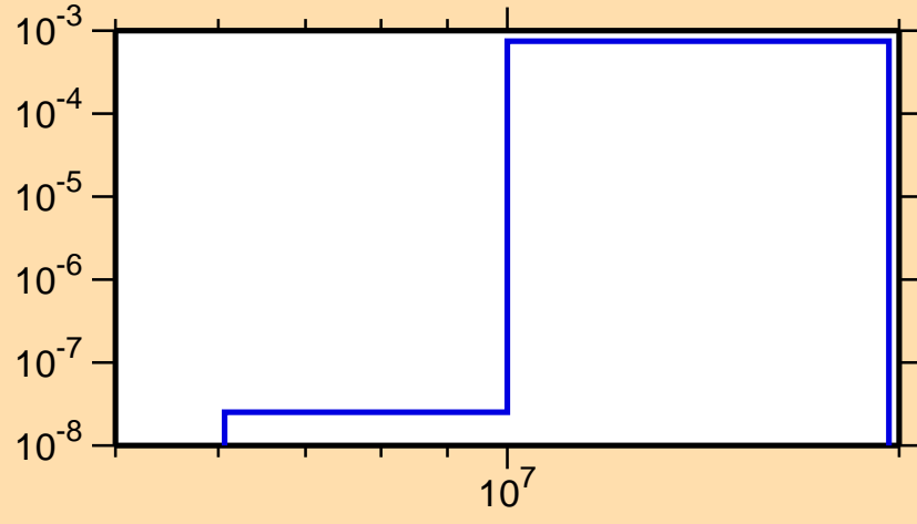
\sigma vs. E for ^{232}\text{Np}(n,d)
