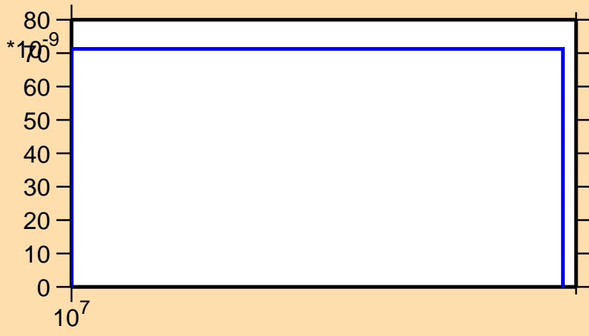
\sigma vs. E for ^{232}\text{Np}(n,2np)
