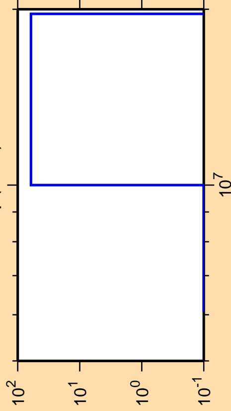
\Delta\sigma/\sigma vs. E for ^{232}\text{Np}(n,\text{nd})
