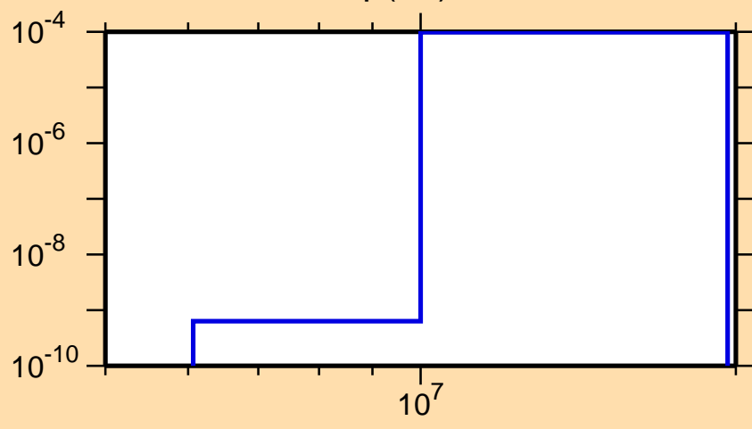
\sigma vs. E for ^{232}\text{Np}(n,t)
