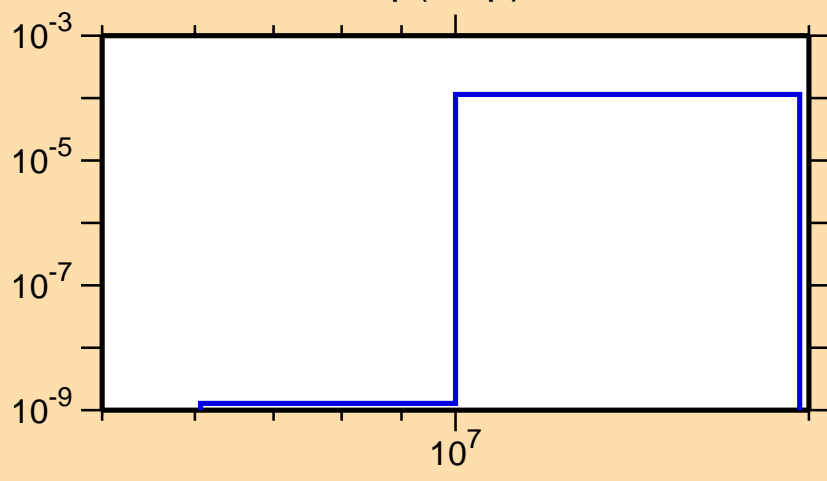
\sigma vs. E for ^{232}\text{Np}(n,np)
