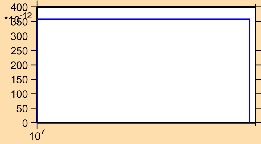
\sigma vs. E for ^{232}\text{Np}(n,\text{He3})
