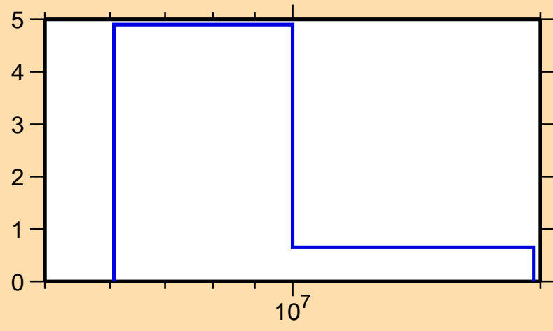
\Delta\sigma/\sigma vs. E for ^{232}\text{Np}(n,\text{el.})
