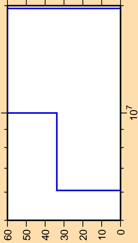
\Delta\sigma/\sigma vs. E for ^{232}\text{Np}(n,t)
