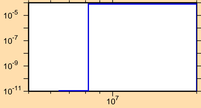
\sigma vs. E for ^{232}\text{Np}(n,t)
