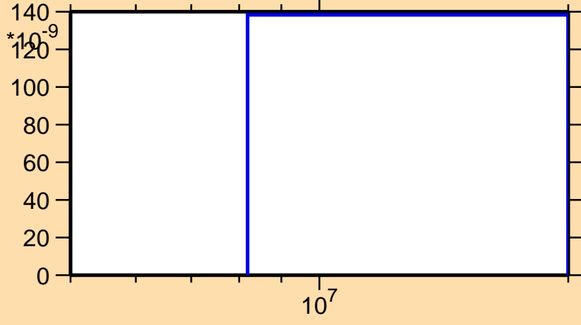
\sigma vs. E for ^{232}\text{Np}(n,nd)
