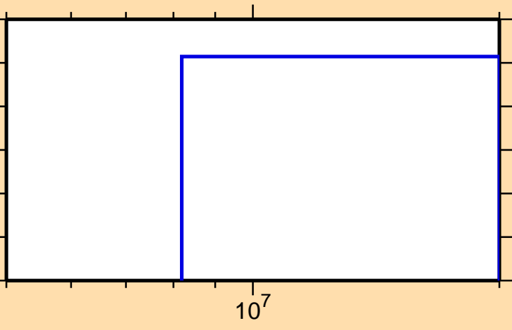
\sigma vs. E for ^{232}\text{Np} (mt 34)
