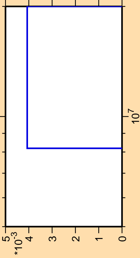
\Delta\sigma/\sigma vs. E for ^{232}\text{Np} (mt 34)
