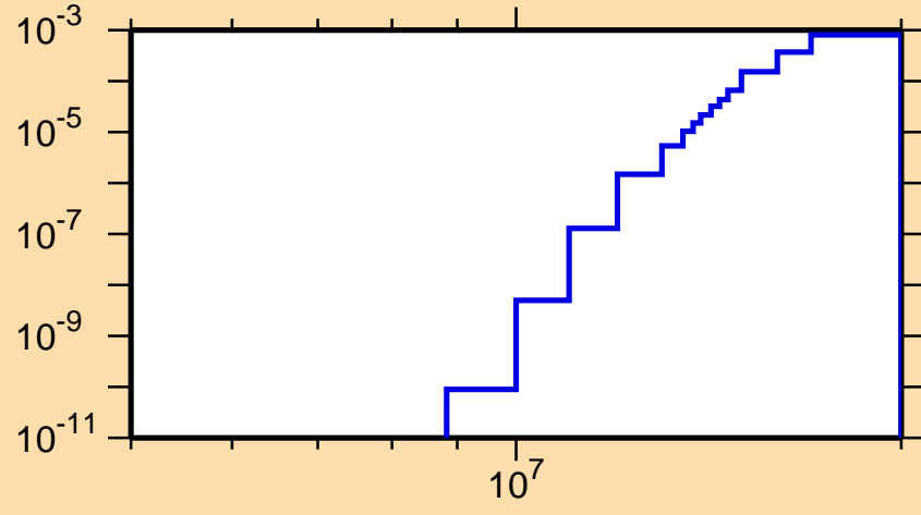
\sigma vs. E for ^{233}\text{Np}(n,t)
