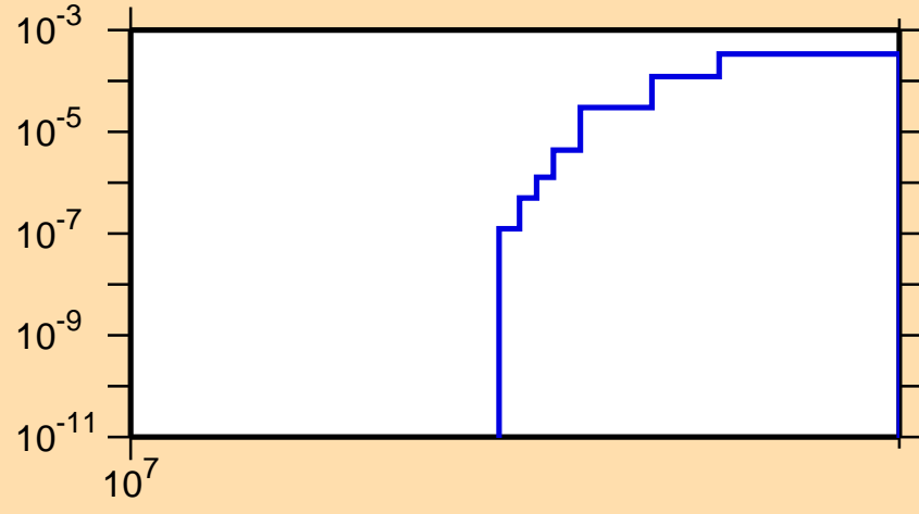
\sigma vs. E for ^{233}\text{Np}(n,3n\alpha)
