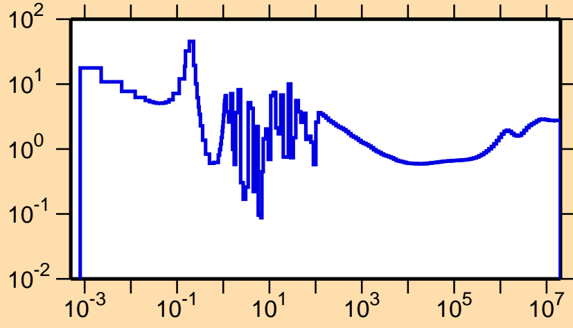
\sigma vs. E for ^{233}\text{Np}(n,f)
