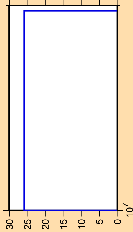
\Delta\sigma/\sigma vs. E for ^{233}\text{Np} (mt 45)
