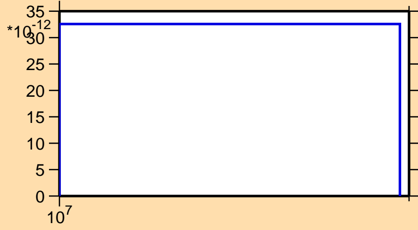
\sigma vs. E for ^{233}\text{Np} (mt 45)
