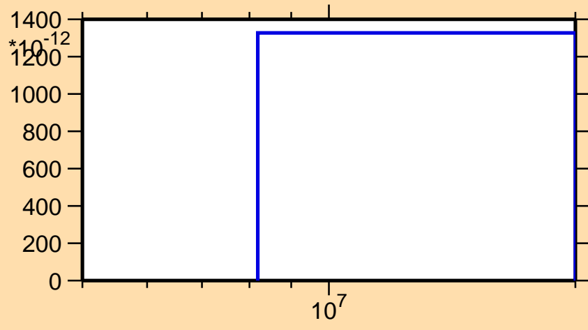
\sigma vs. E for ^{233}\text{Np}(n,2np)
