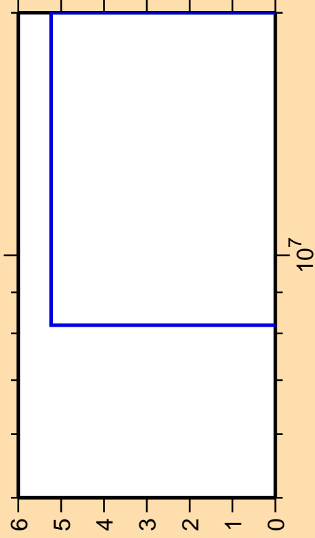
\Delta\sigma/\sigma vs. E for ^{233}\text{Np}(n,\text{He3})
