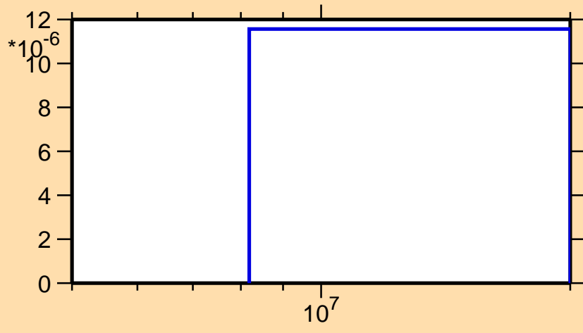
\sigma vs. E for ^{233}\text{Np}(n,3n\alpha)
