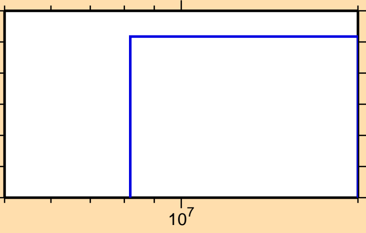
\sigma vs. E for ^{233}\text{Np}(n,t)
