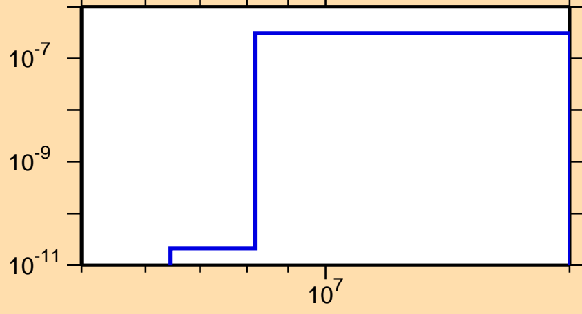
\sigma vs. E for ^{233}\text{Np}(n,2n\alpha)
