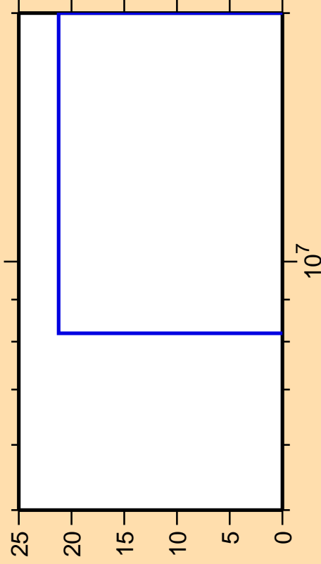
\Delta\sigma/\sigma vs. E for ^{233}\text{Np}(\text{mt } 45)
