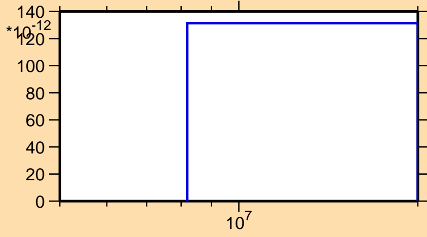
\sigma vs. E for ^{233}\text{Np}(\text{mt117})
