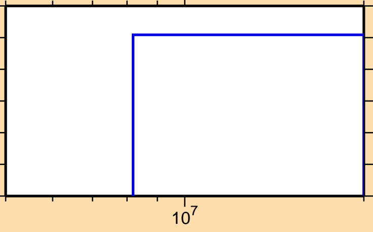
\sigma vs. E for ^{233}\text{Np}(n,nt)
