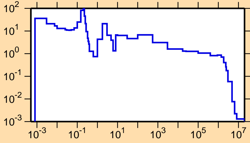
\sigma vs. E for ^{233}\text{Np}(n,\gamma)
