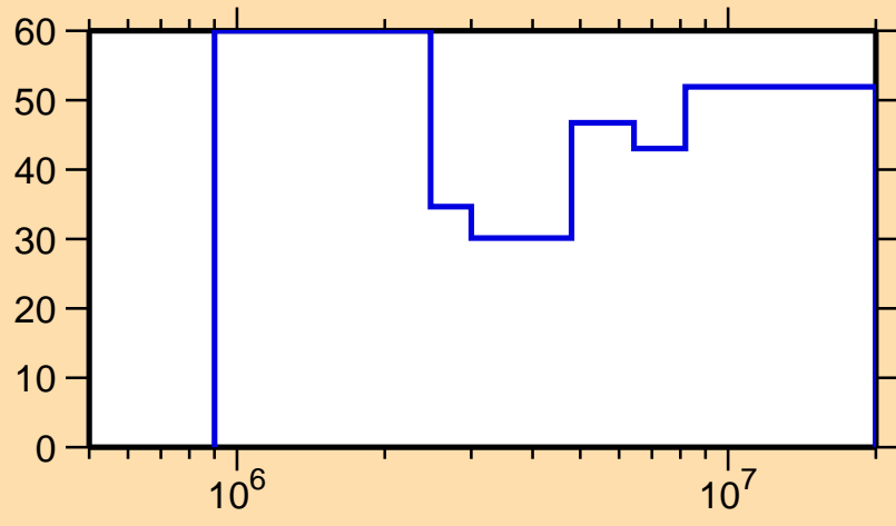
\Delta\sigma/\sigma vs. E for ^{233}\text{Np}(n,n\text{cont.})
