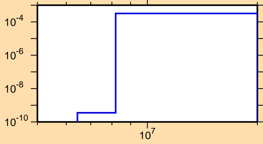
\sigma vs. E for ^{233}\text{Np}(n,d)
