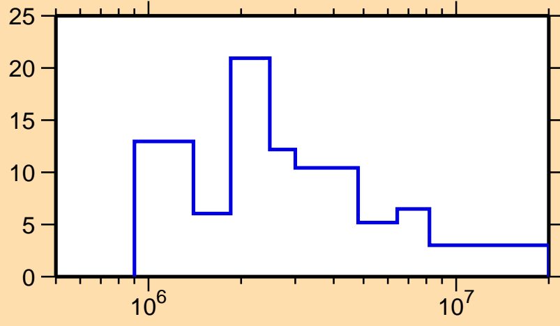
\Delta\sigma/\sigma vs. E for ^{233}\text{Np}(n,f)
