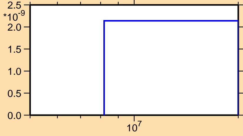
\sigma vs. E for ^{233}\text{Np}(n,\text{nd})
