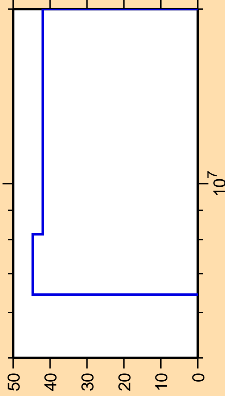
\Delta\sigma/\sigma vs. E for ^{233}\text{Np}(n,n_1)
