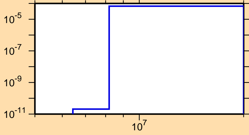
\sigma vs. E for ^{233}\text{Np}(n,np)
