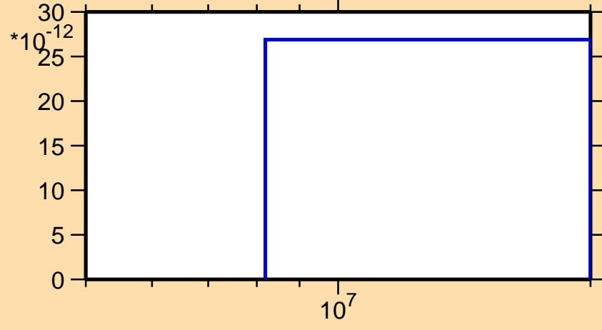
\sigma vs. E for ^{233}\text{Np}(\text{mt } 45)
