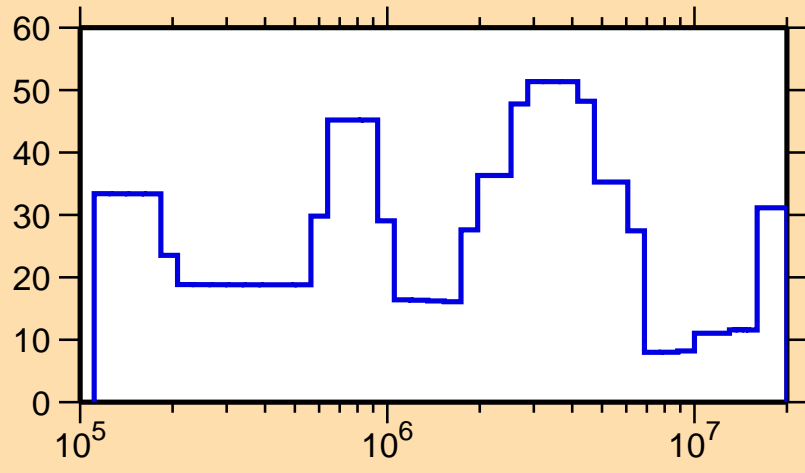
\Delta\sigma/\sigma vs. E for ^{234}\text{Np}(n,\text{el.})
