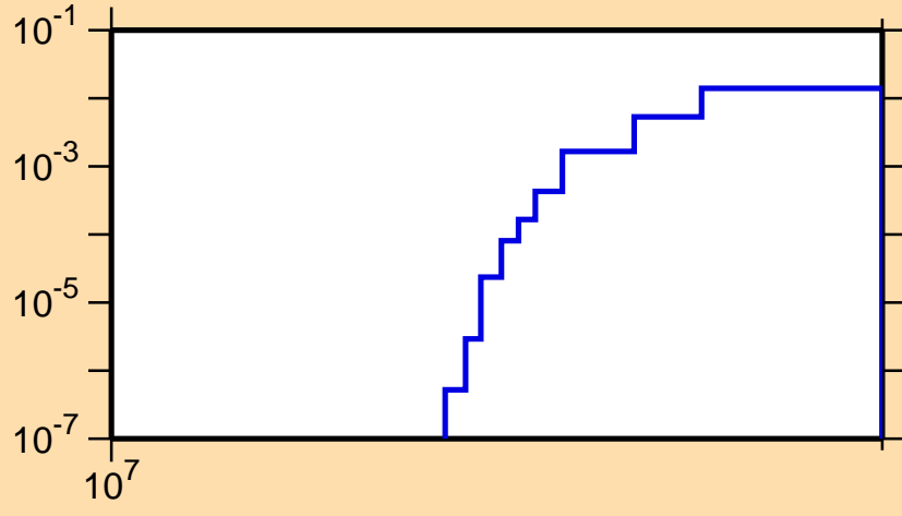
\sigma vs. E for ^{234}\text{Np}(n,3n)
