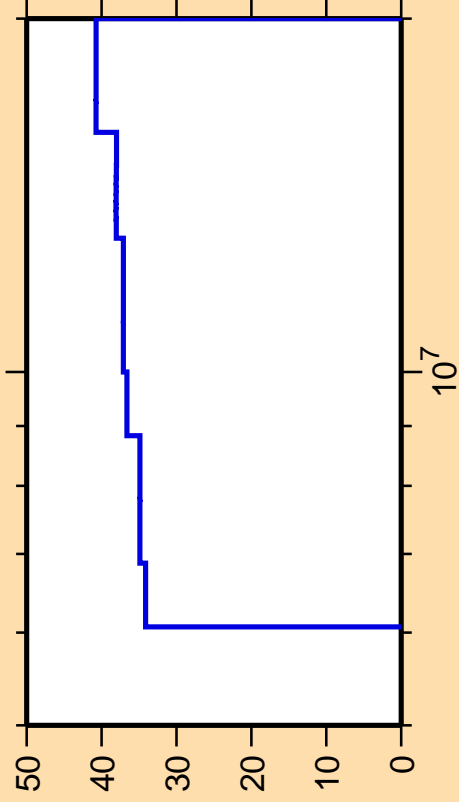
\Delta\sigma/\sigma vs. E for ^{234}\text{Np}(n,p)
