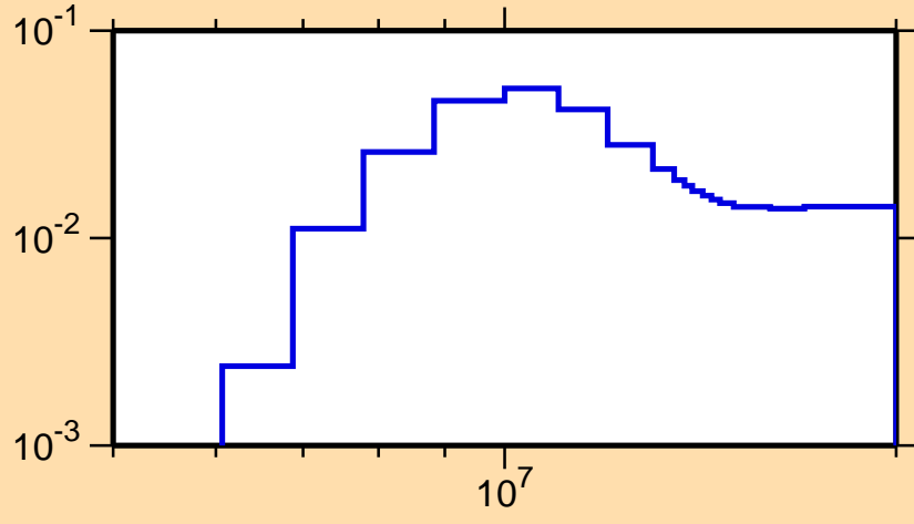
\sigma vs. E for ^{234}\text{Np}(n,2n)
