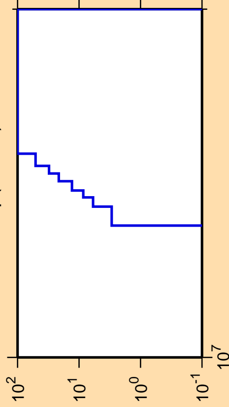
\Delta\sigma/\sigma vs. E for ^{234}\text{Np}(\text{mt117})
