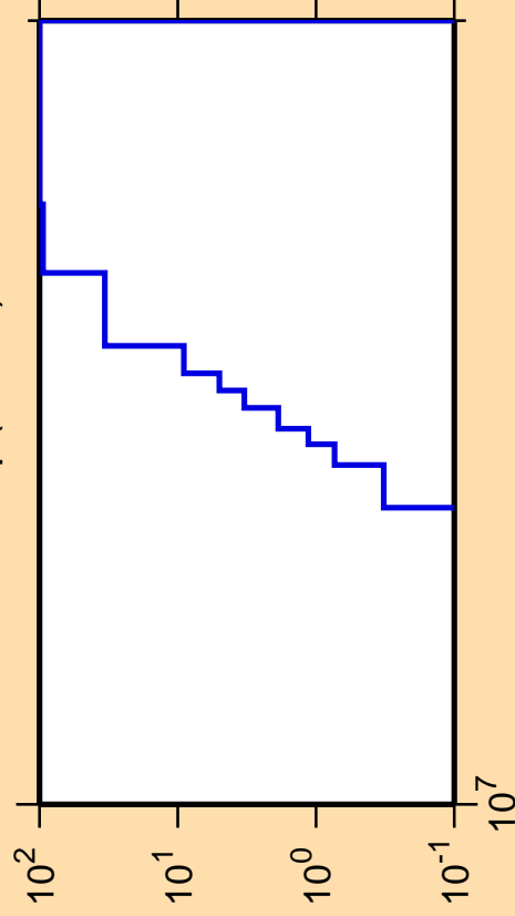
\Delta\sigma/\sigma vs. E for ^{234}\text{Np}(\text{mt } 45)
