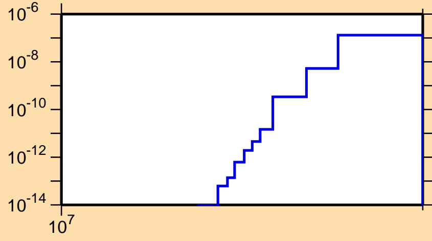
\sigma vs. E for ^{234}\text{Np}(n,nt)
