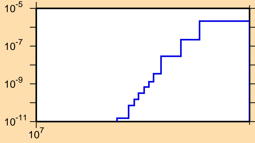
\sigma vs. E for ^{234}\text{Np}(n,\text{nd})
