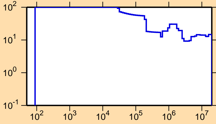
\Delta\sigma/\sigma vs. E for ^{234}\text{Np}(n,\text{nonel.})
