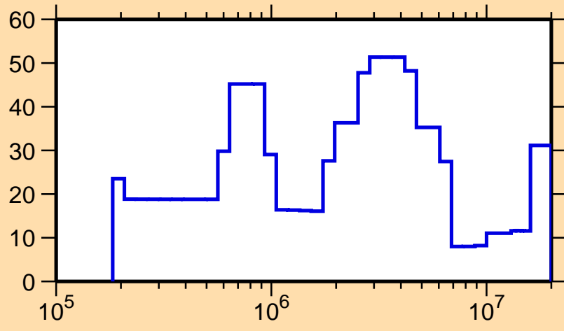
\Delta\sigma/\sigma vs. E for ^{234}\text{Np}(n,el.)
