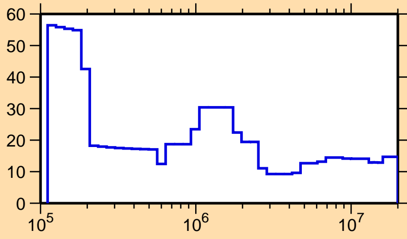
\Delta\sigma/\sigma vs. E for ^{234}\text{Np}(n,\text{nonel.})
