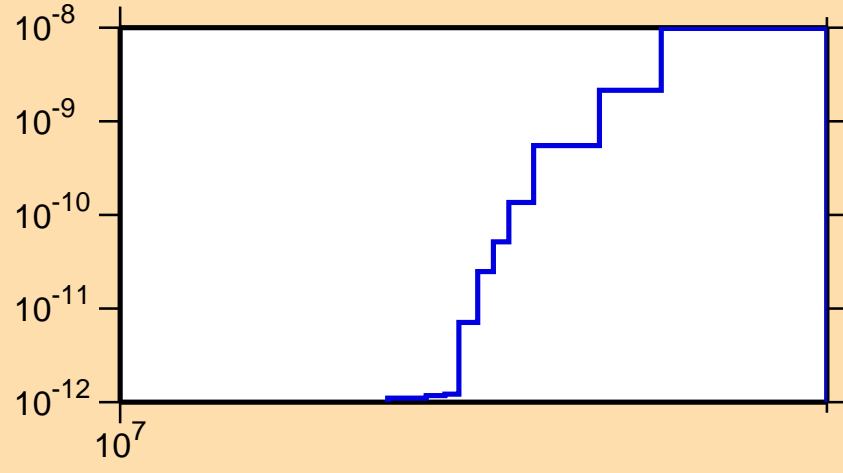
\sigma vs. E for ^{234}\text{Np}(n,3n\alpha)
