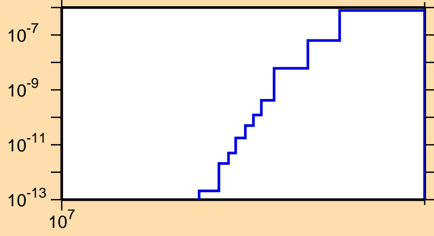
\sigma vs. E for ^{234}\text{Np}(n,2np)
