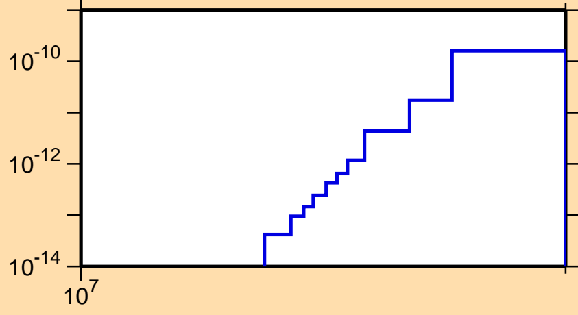
\sigma vs. E for ^{234}\text{Np}(\text{mt } 45)
