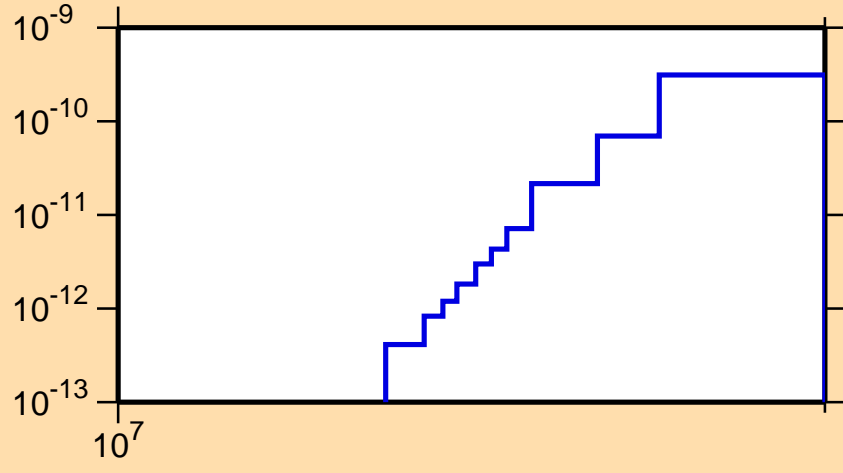
\sigma vs. E for ^{234}\text{Np}(\text{mt117})
