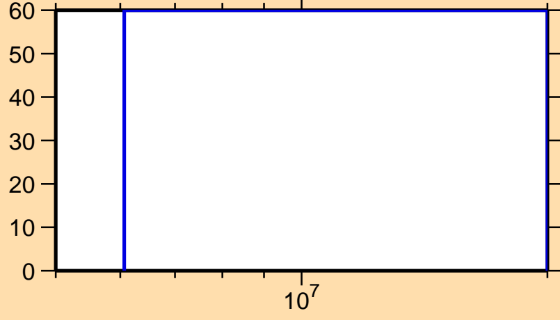
\Delta\sigma/\sigma vs. E for ^{234}\text{Np}(n,2n)
