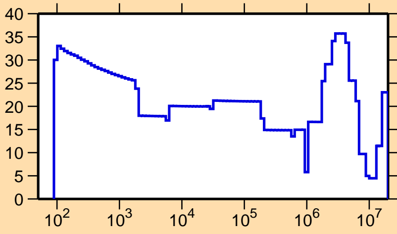
\Delta\sigma/\sigma vs. E for ^{234}\text{Np}(n,\text{tot.})
