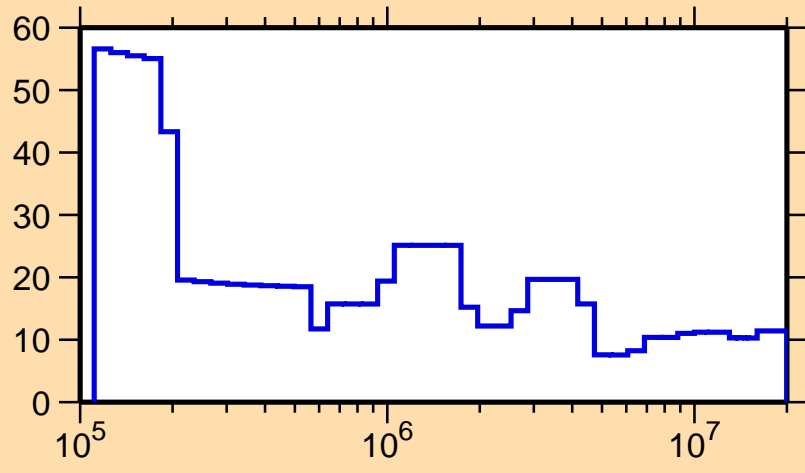
\Delta\sigma/\sigma vs. E for ^{234}\text{Np}(n,f)
