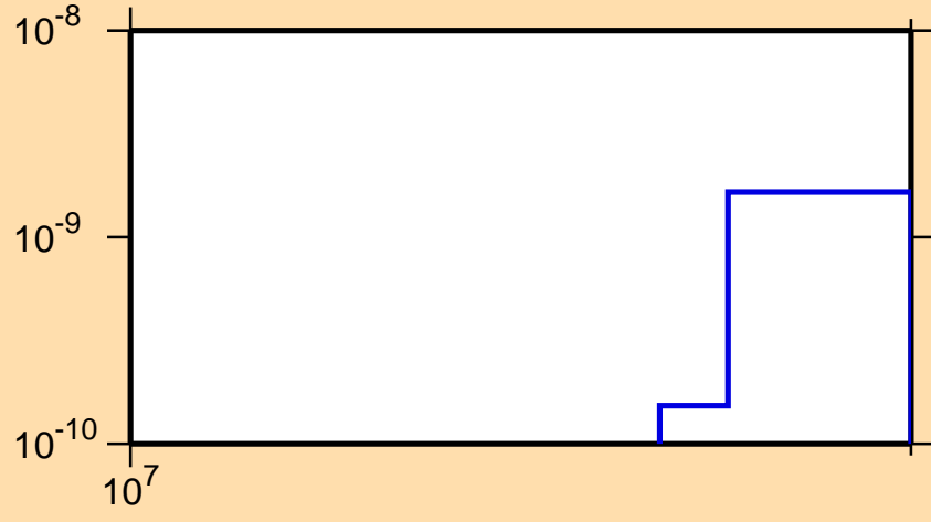
\sigma vs. E for ^{234}\text{Np}(n,\text{He3})
