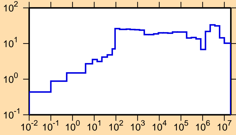
\Delta\sigma/\sigma vs. E for ^{234}\text{Np}(n,tot.)
