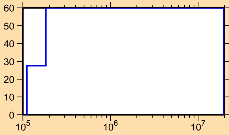
\Delta\sigma/\sigma vs. E for ^{234}\text{Np}(n,n_1)
