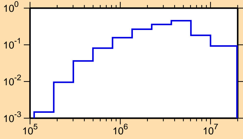
\sigma vs. E for ^{234}\text{Np}(n,n\text{cont.})
