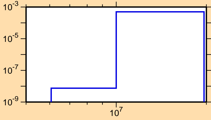
\sigma vs. E for ^{234}\text{Np}(n,d)
