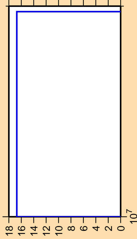
\Delta\sigma/\sigma vs. E for ^{234}\text{Np} (mt 45)
