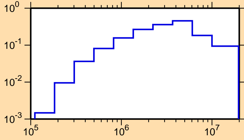
\sigma vs. E for ^{234}\text{Np}(n,\text{inel.})
