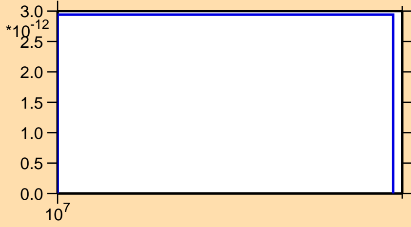
\sigma vs. E for ^{234}\text{Np} (mt 45)
