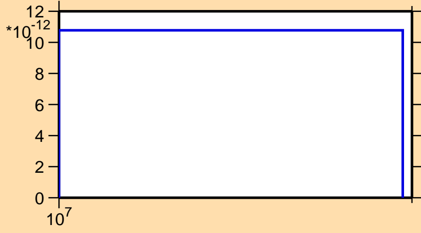
\sigma vs. E for ^{234}\text{Np}(\text{mt117})
