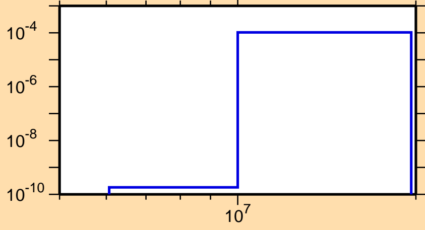
\sigma vs. E for ^{234}\text{Np}(n,t)
