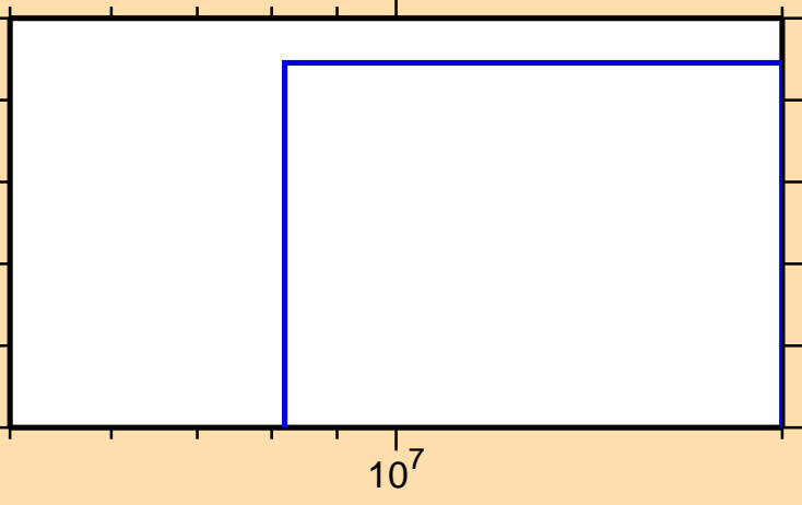
\sigma vs. E for ^{234}\text{Np}(n,\text{He3})
