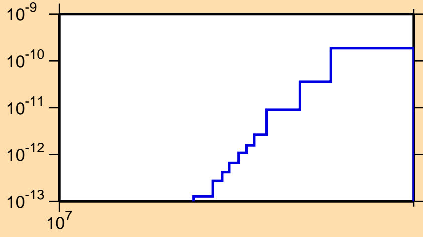
\sigma vs. E for ^{235}\text{Np}(\text{mt117})
