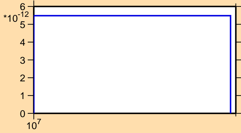
\sigma vs. E for ^{235}\text{Np}(\text{mt117})
