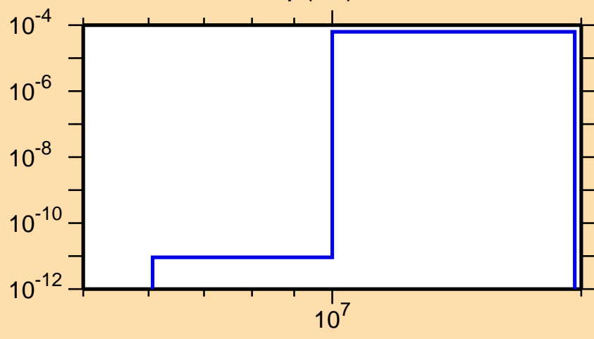
\sigma vs. E for ^{235}\text{Np}(n,t)
