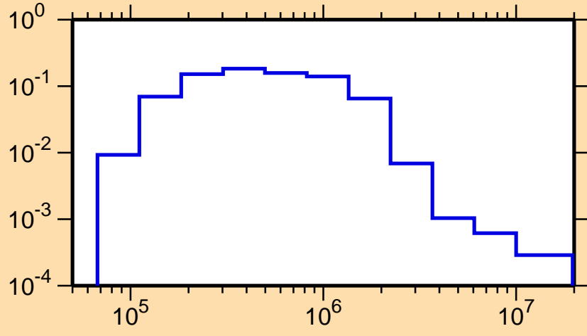
\sigma vs. E for ^{235}\text{Np}(n,n_3)
