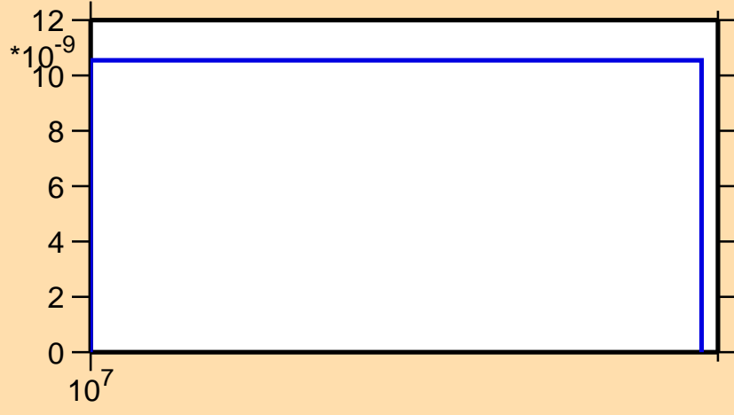
\sigma vs. E for ^{235}\text{Np}(n,\text{nd})
