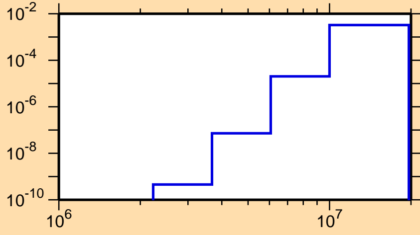
\sigma vs. E for ^{235}\text{Np}(n,p)
