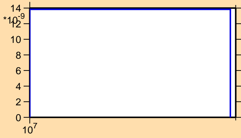
\sigma vs. E for ^{235}\text{Np}(n,3n\alpha)
