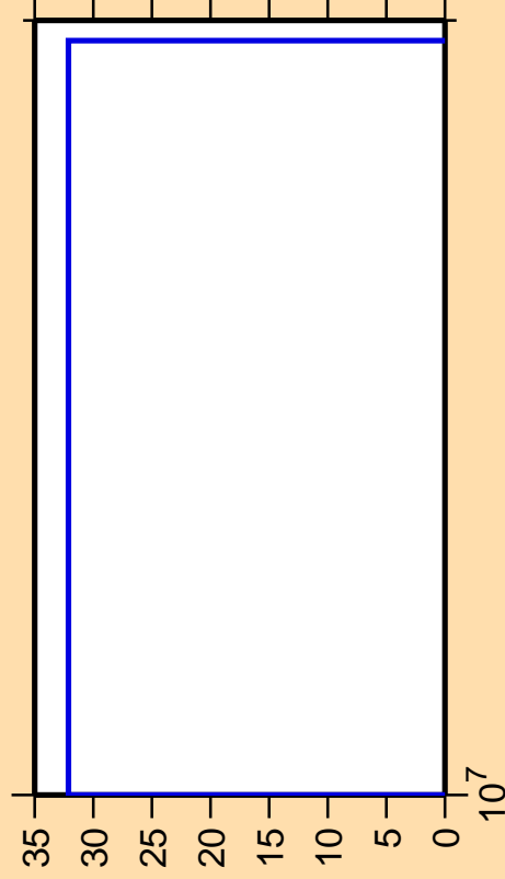
\Delta\sigma/\sigma vs. E for ^{235}\text{Np}(\text{mt117})
