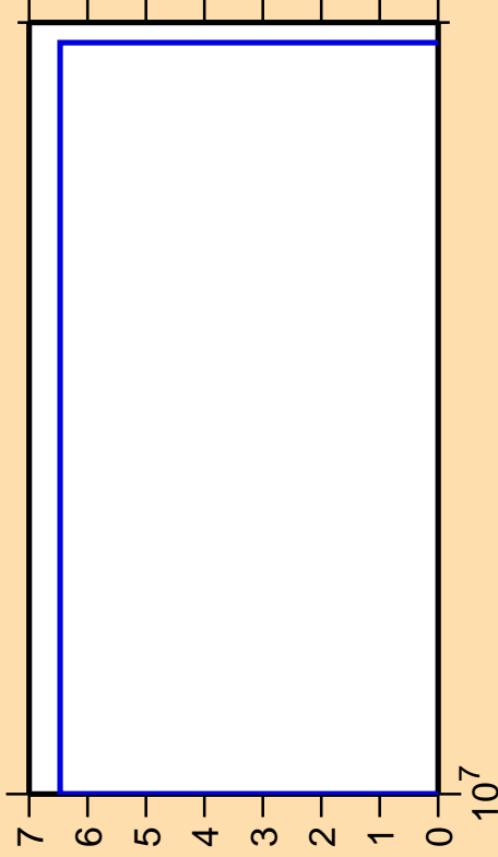
\Delta\sigma/\sigma vs. E for ^{235}\text{Np}(\text{mt } 45)
