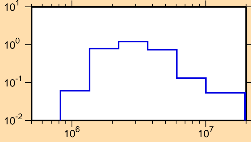
\sigma vs. E for ^{235}\text{Np}(n,n\text{cont.})
