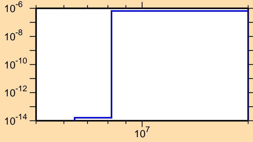
\sigma vs. E for ^{235}\text{Np}(n,2n\alpha)
