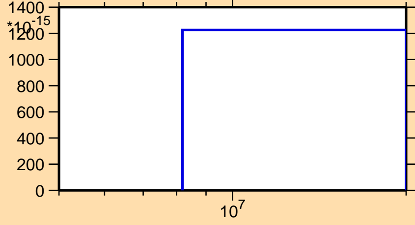
\sigma vs. E for ^{235}\text{Np}(\text{mt } 45)
