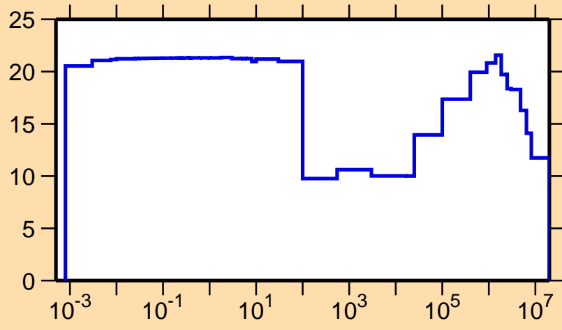
\Delta\sigma/\sigma vs. E for ^{235}\text{Np}(n,el.)
