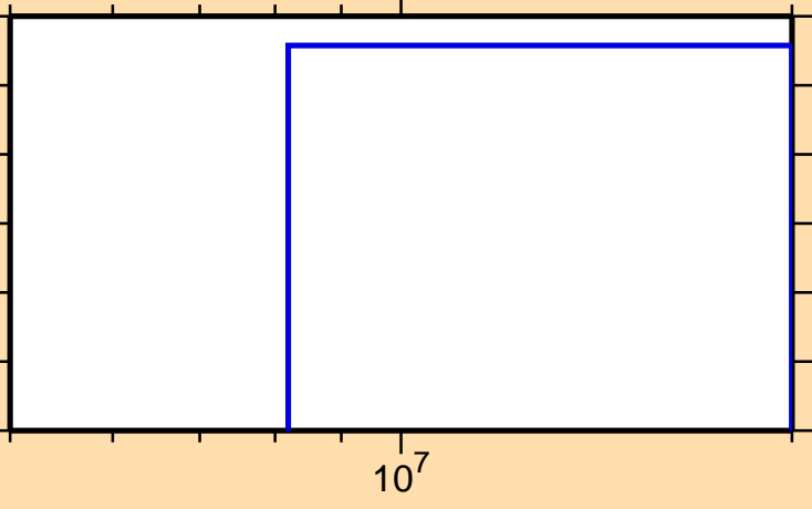
\sigma vs. E for ^{235}\text{Np}(n,3n\alpha)
