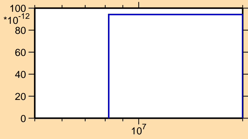
\sigma vs. E for ^{235}\text{Np}(n,p\alpha)
