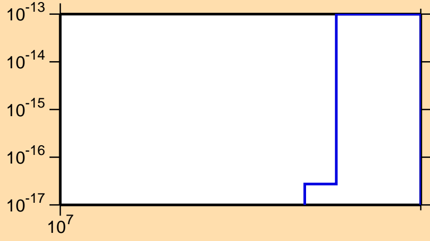
\sigma vs. E for ^{236}\text{Np} (mt 11)
