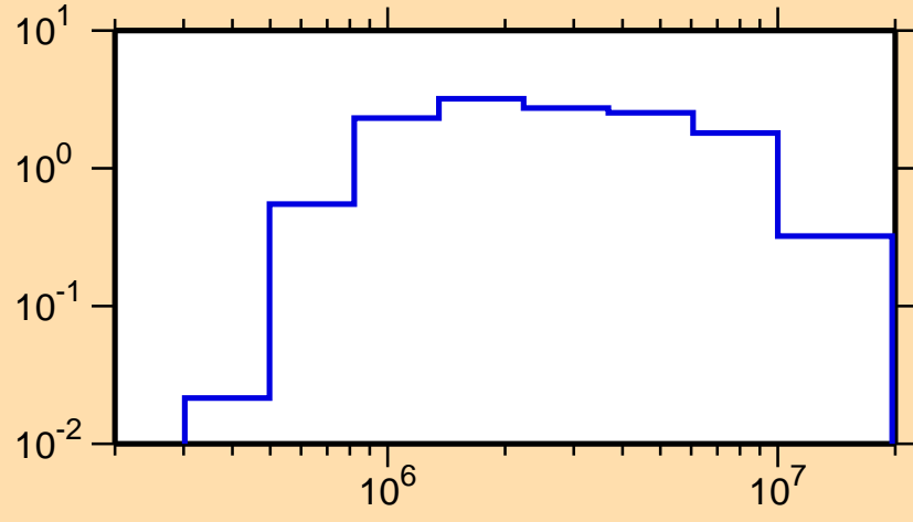
\sigma vs. E for ^{236}\text{Np}(n,n\text{cont.})
