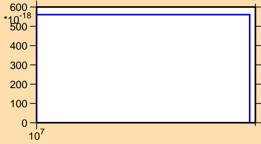
\sigma vs. E for ^{236}\text{Np} (mt 11)
