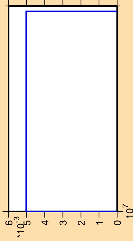
\Delta\sigma/\sigma vs. E for ^{236}\text{Np} (mt 11)
