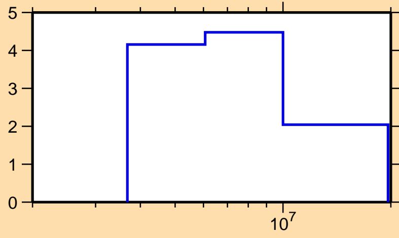
\Delta\sigma/\sigma vs. E for ^{236}\text{Np}(n,\text{nonel.})
