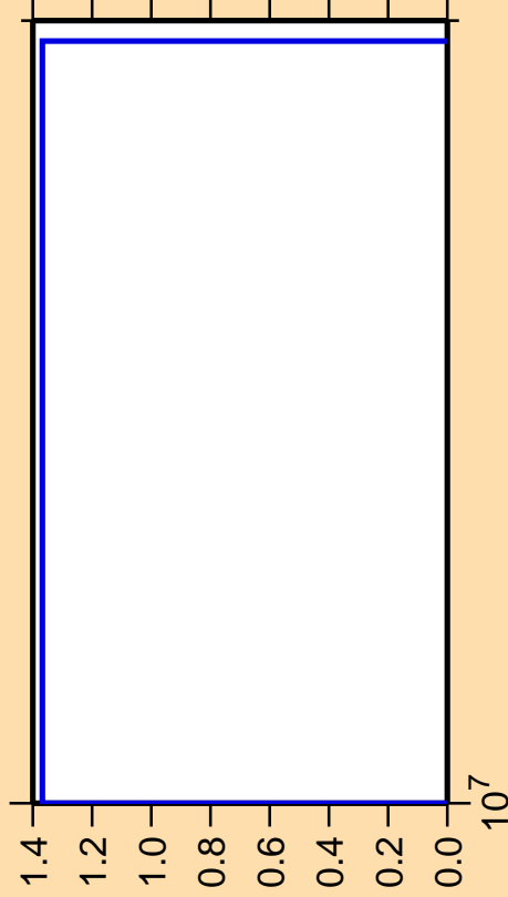
\Delta\sigma/\sigma vs. E for ^{236}\text{Np} (mt 45)
