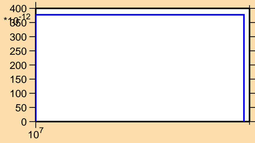
\sigma vs. E for ^{236}\text{Np}(n,3n\alpha)
