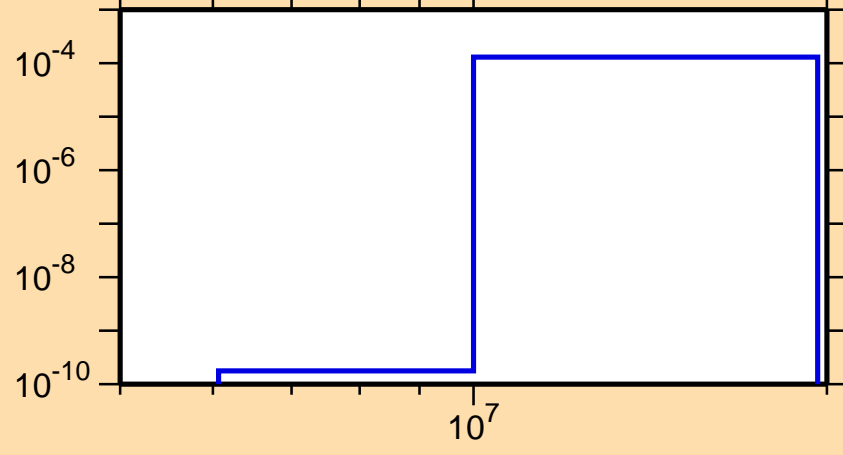
\sigma vs. E for ^{236}\text{Np}(n,np)
