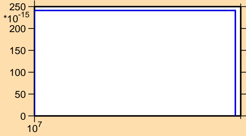
\sigma vs. E for ^{236}\text{Np} (mt 45)
