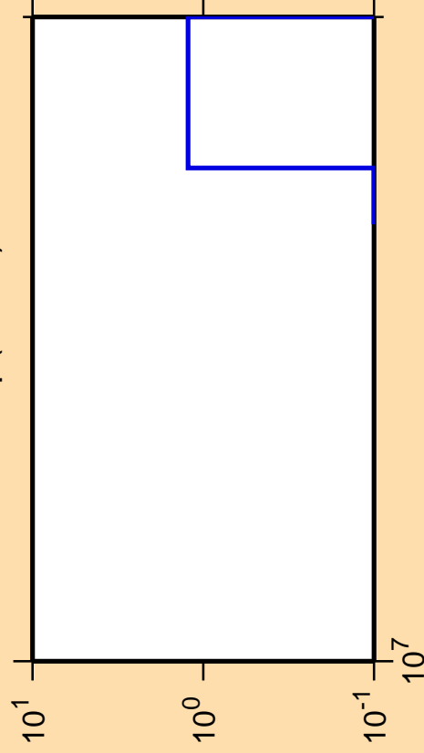
\Delta\sigma/\sigma vs. E for ^{236}\text{Np} (mt 11)
