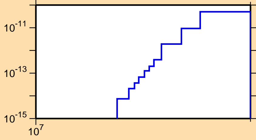
\sigma vs. E for ^{236}\text{Np}(\text{mt } 45)
