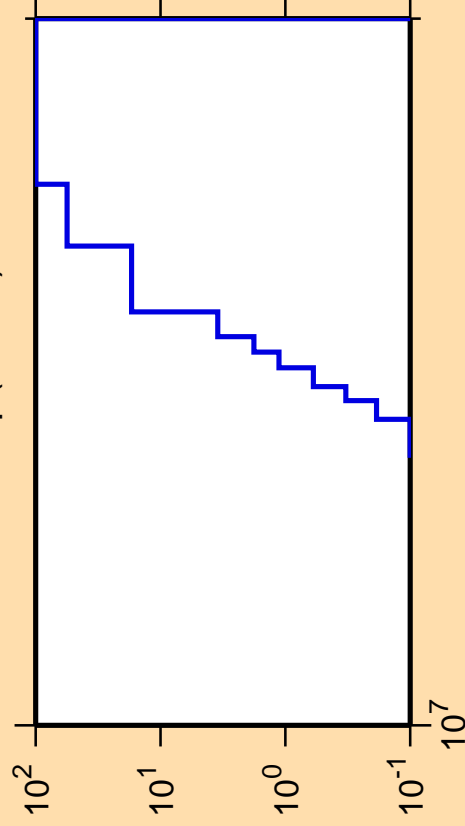
\Delta\sigma/\sigma vs. E for ^{236}\text{Np}(\text{mt } 45)
