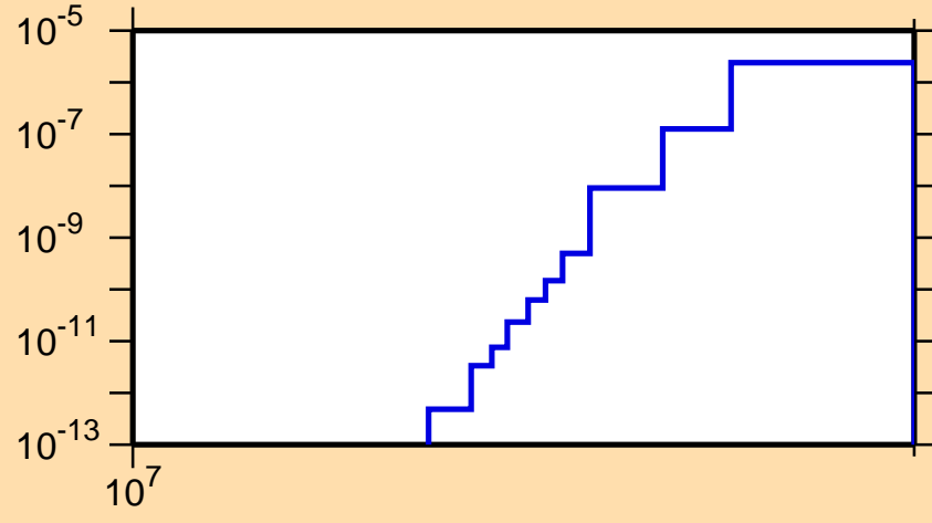
\sigma vs. E for ^{236}\text{Np}(n,nt)
