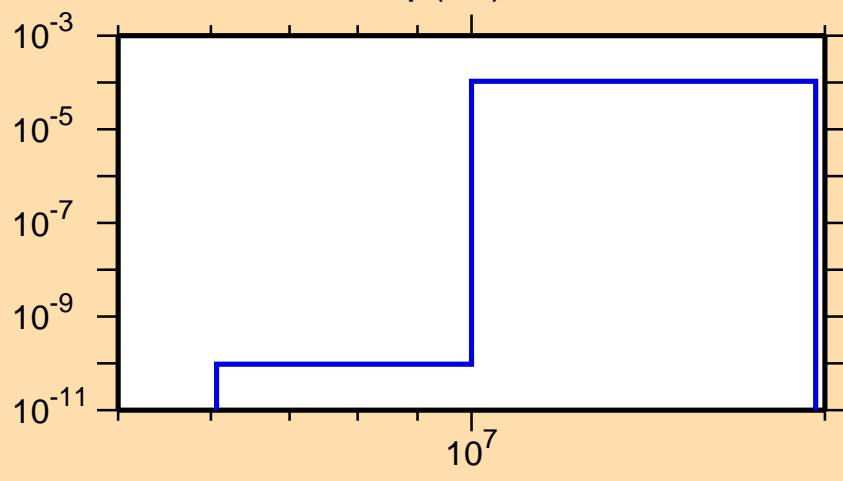
\sigma vs. E for ^{236}\text{Np}(n,t)
